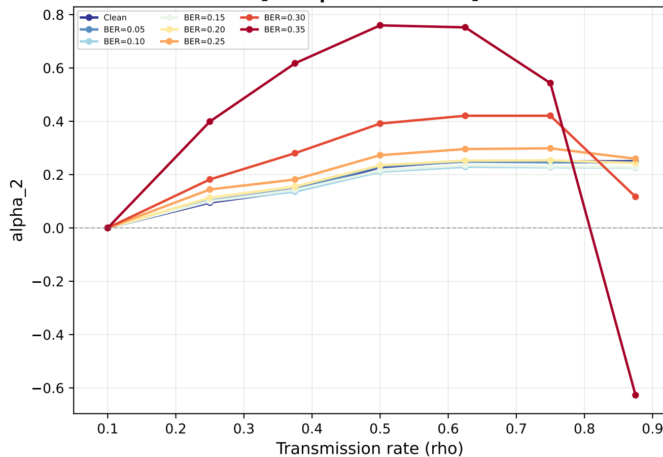
AID: \alpha_2 = (A(\rho) - A(\rho_{\min})) / A(\rho_{\min}) [Fair: per- \rho trained]
