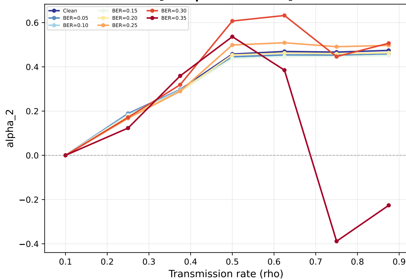
RESISC45: \alpha_2 = (A(\rho) - A(\rho_{\min})) / A(\rho_{\min}) [Fair: per- \rho trained]
