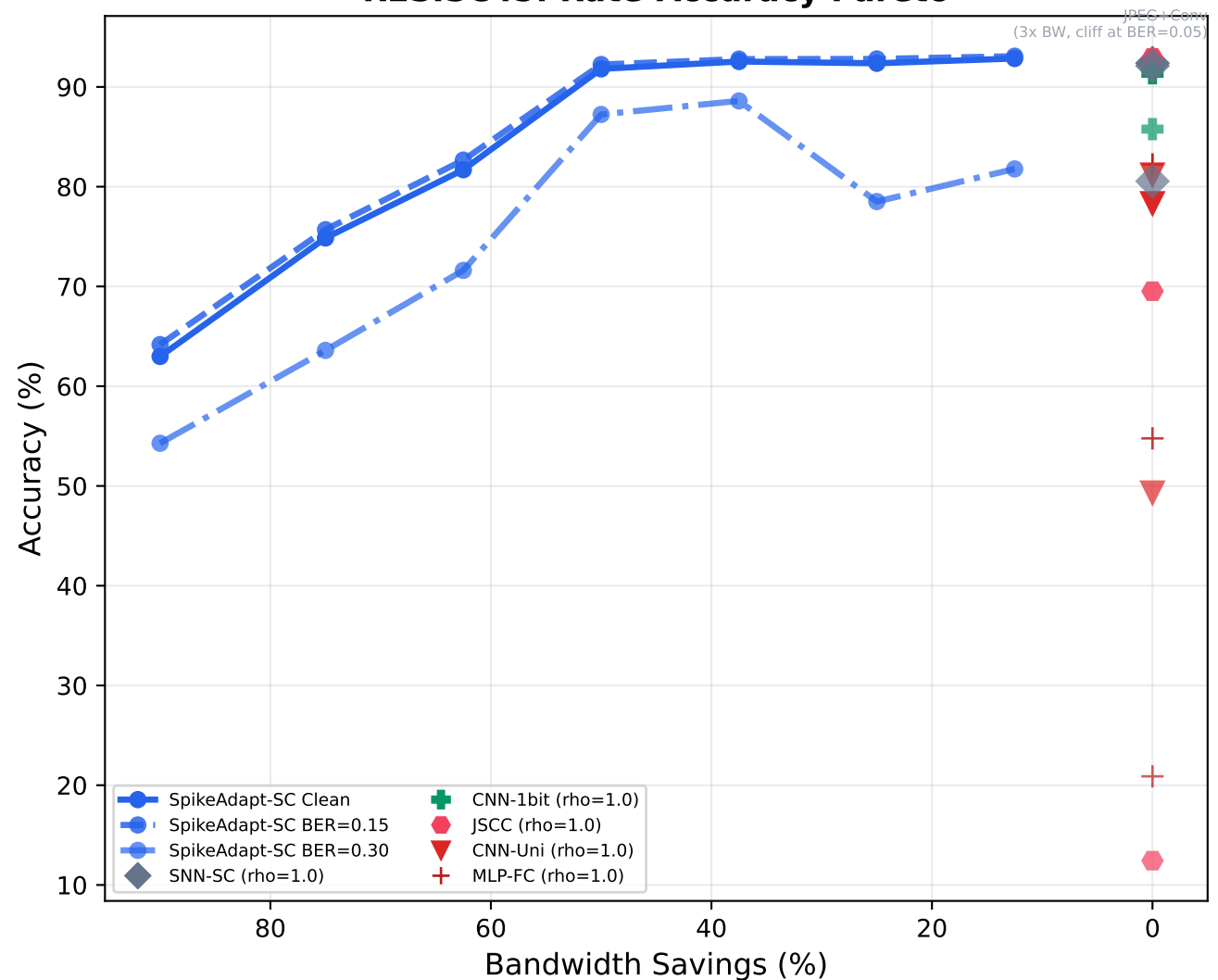
RESISC45: Rate-Accuracy Pareto
