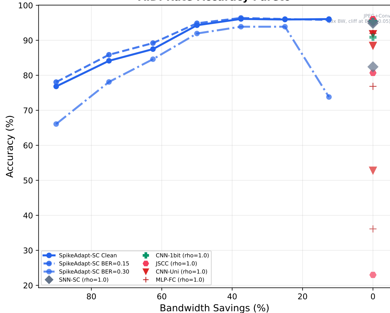
AID: Rate-Accuracy Pareto
