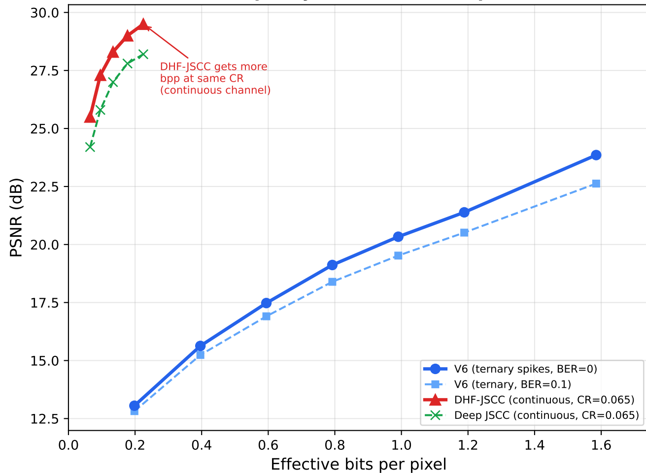
KITTI: Capacity-Normalized Comparison
