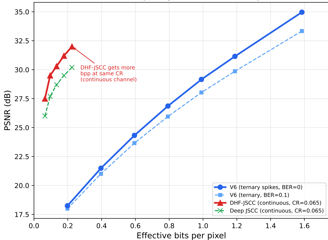
InStereo2K: Capacity-Normalized Comparison
