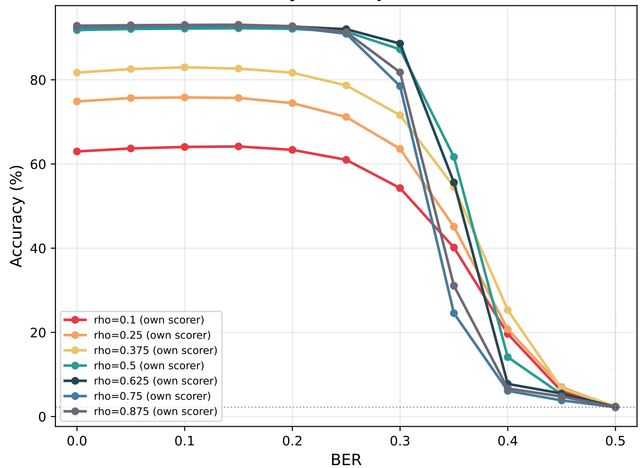
RESISC45: Accuracy vs BER (per-rho trained, FAIR)
