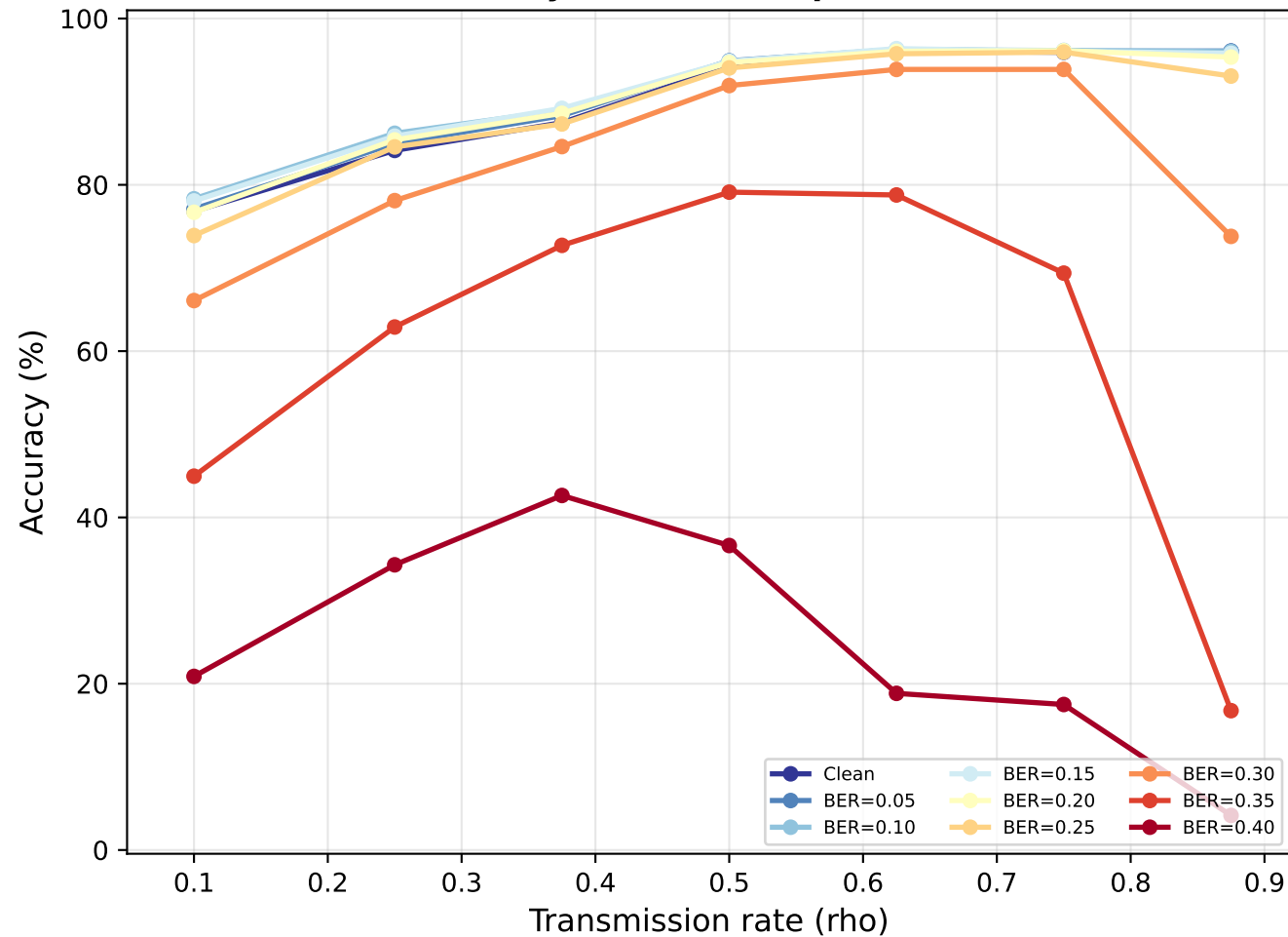
AID: Accuracy vs rho (FAIR, per-rho trained)
