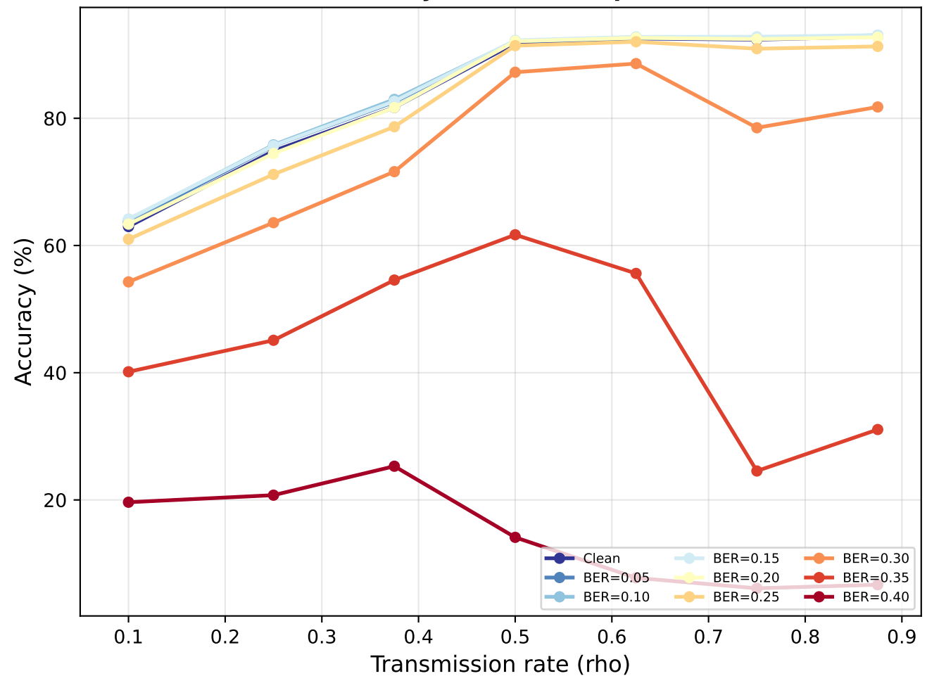
RESISC45: Accuracy vs rho (FAIR, per-rho trained)
