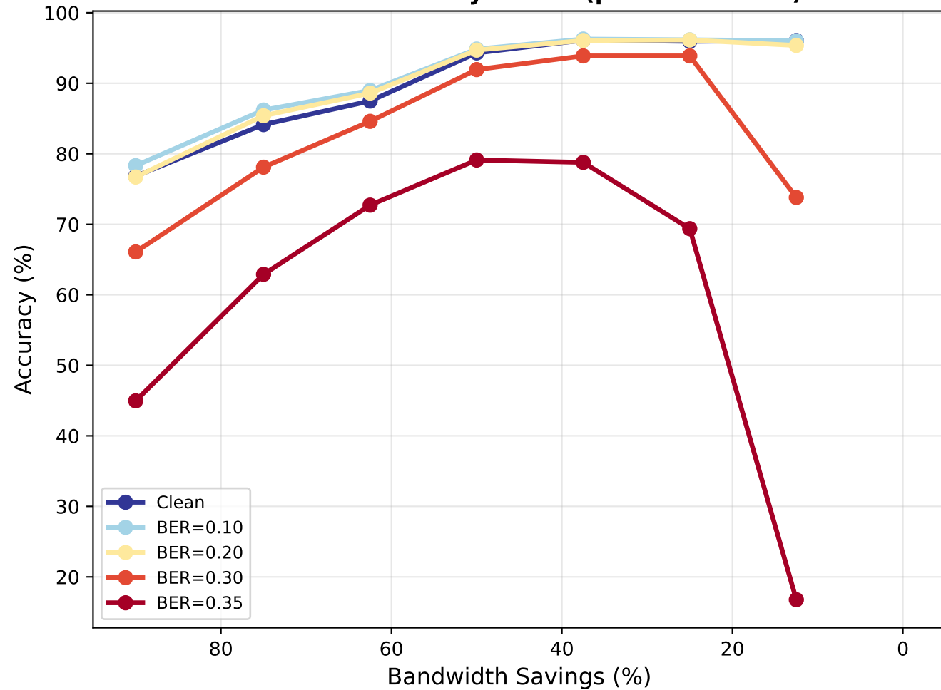
AID: Rate-Accuracy Pareto (per-rho trained)
