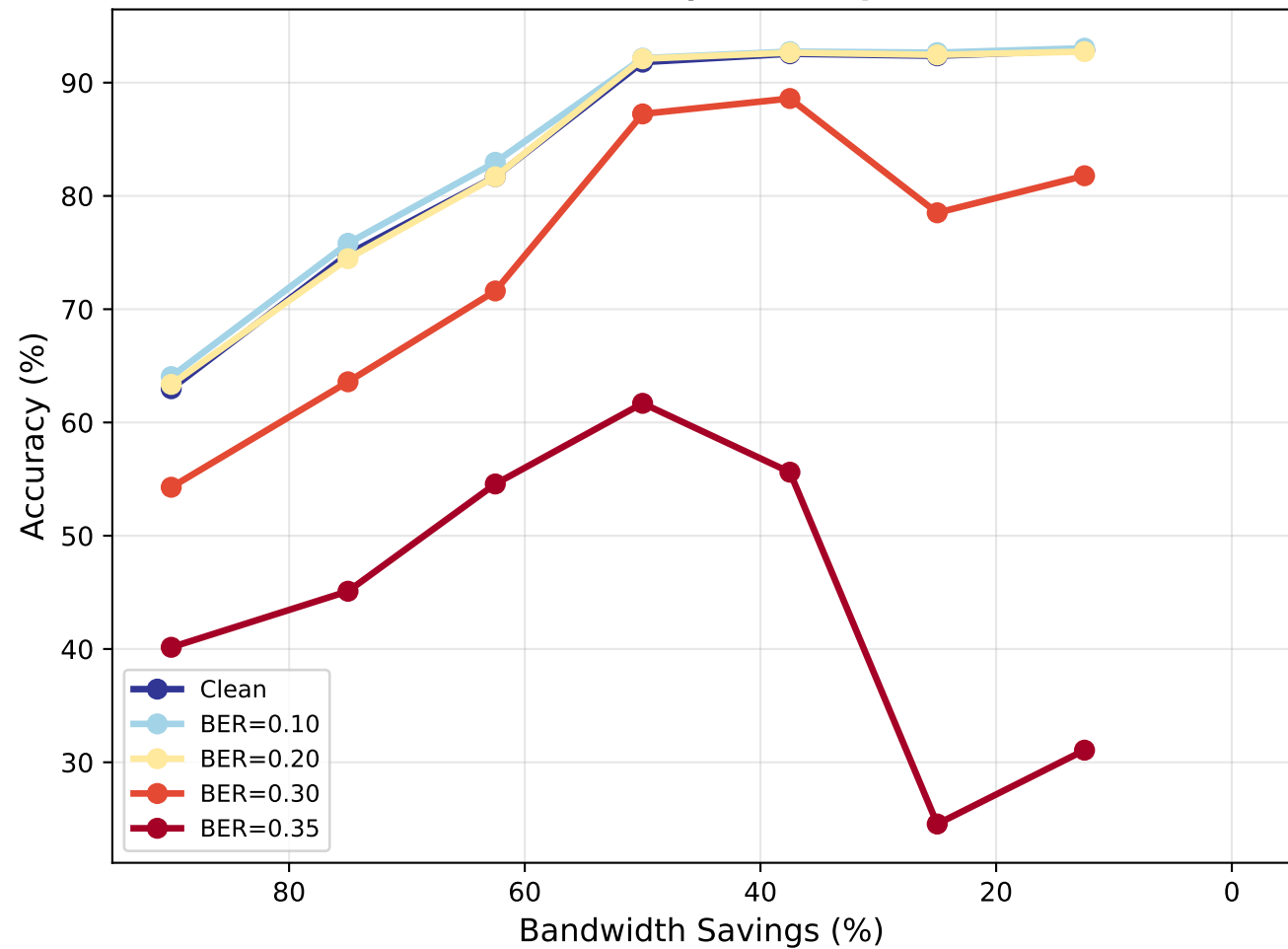
RESISC45: Rate-Accuracy Pareto (per-rho trained)
