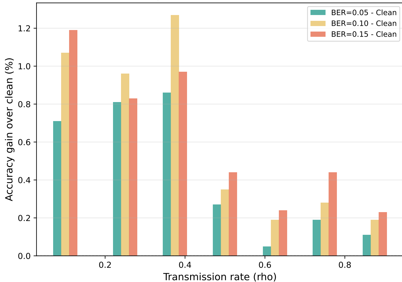
RESISC45: Stochastic Resonance (positive = noise HELPS)
