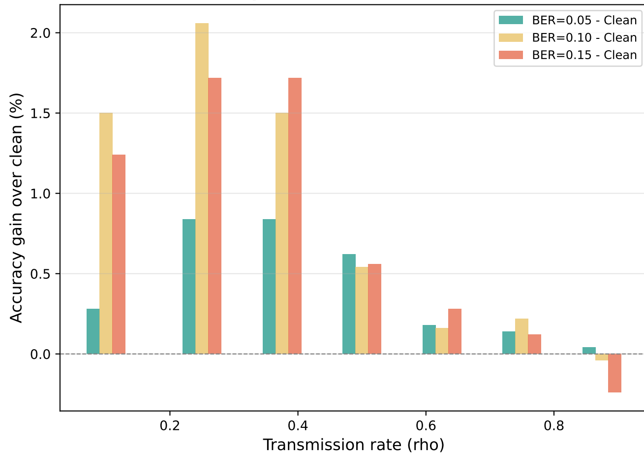
AID: Stochastic Resonance (positive = noise HELPS)
