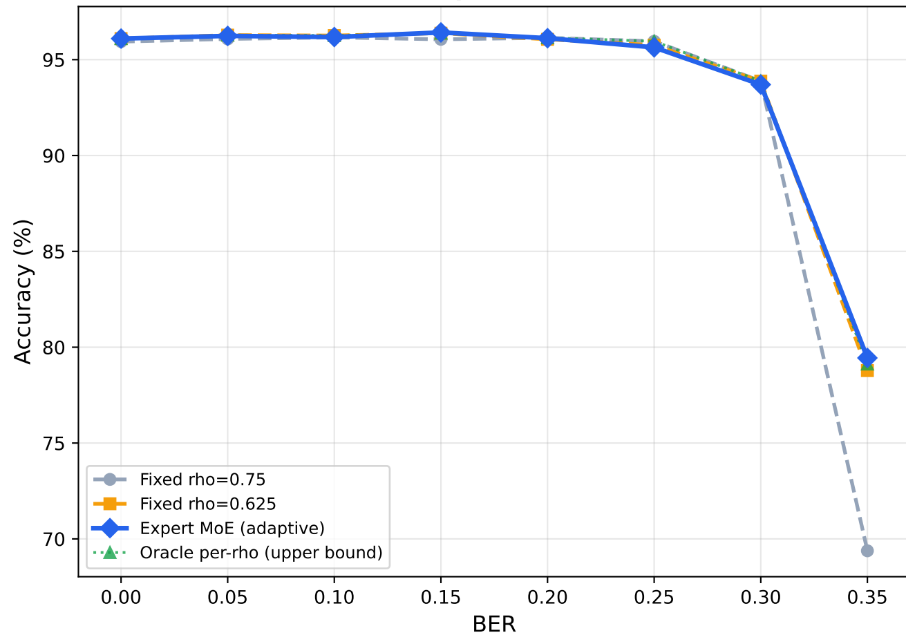
AID: Expert MoE vs Fixed vs Oracle (seed 42, per-rho scorers)
