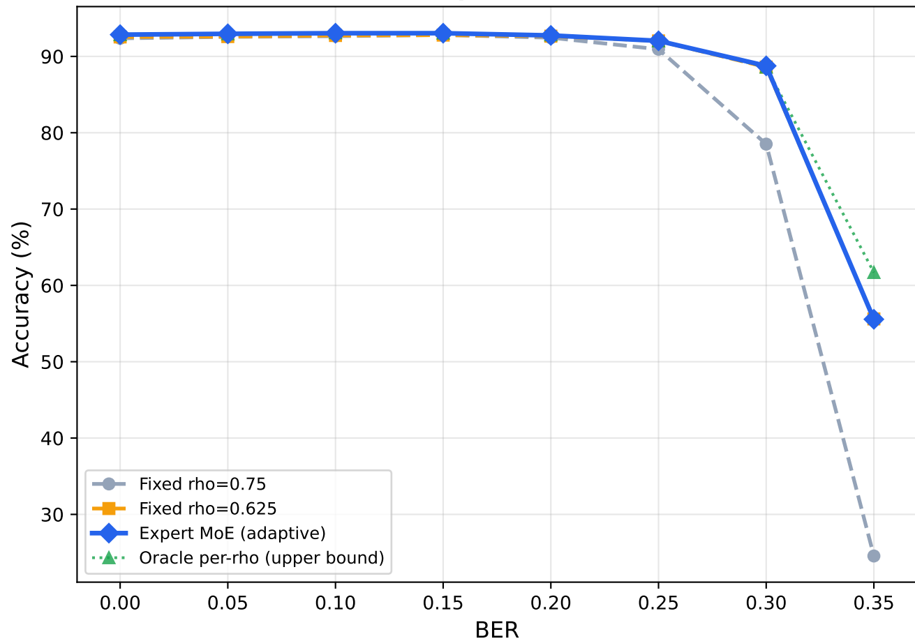
RESISC45: Expert MoE vs Fixed vs Oracle (seed 42, per-rho scorers)
