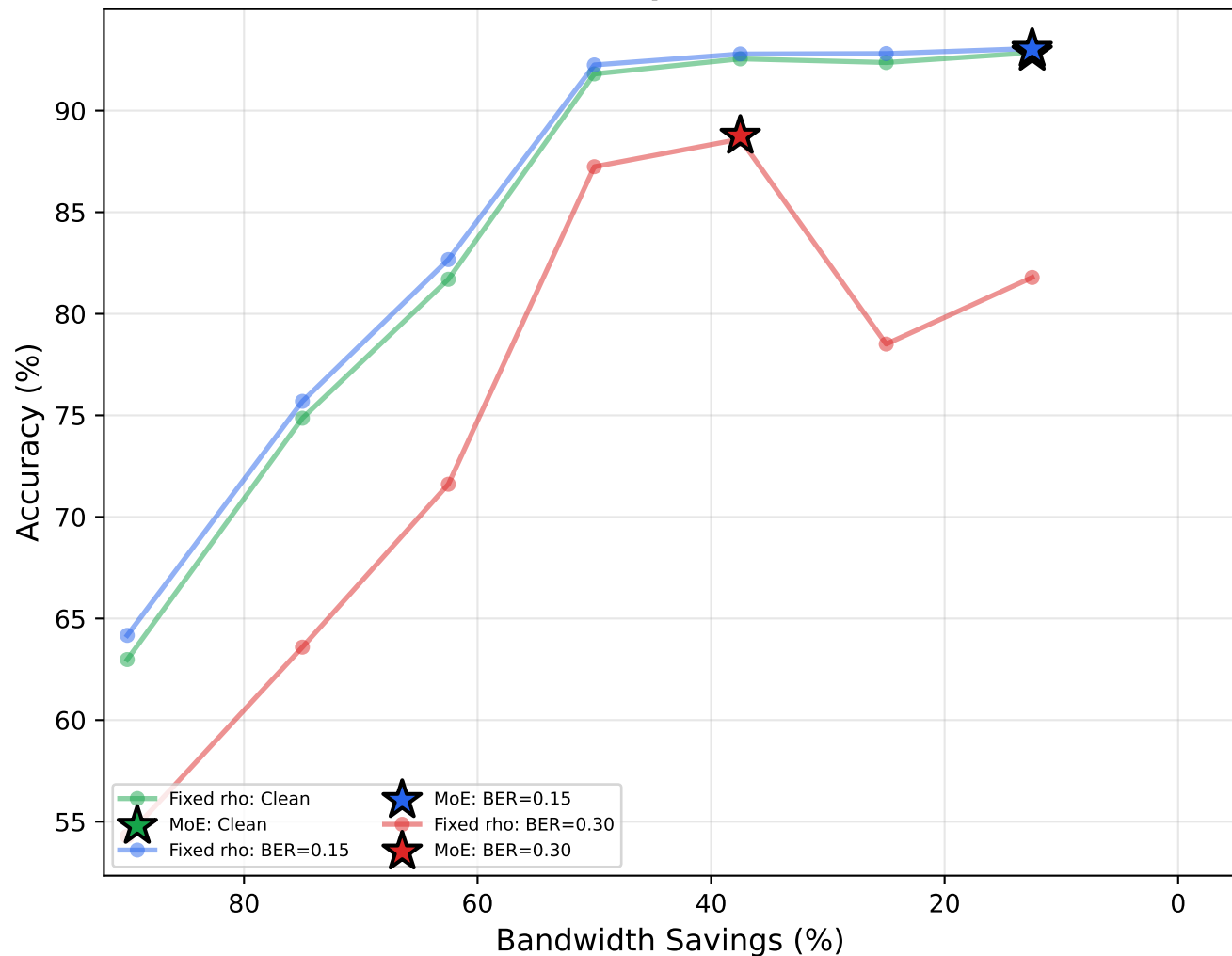
RESISC45: Rate-Accuracy with Adaptive MoE (MoE stars = expert-selected rho)
