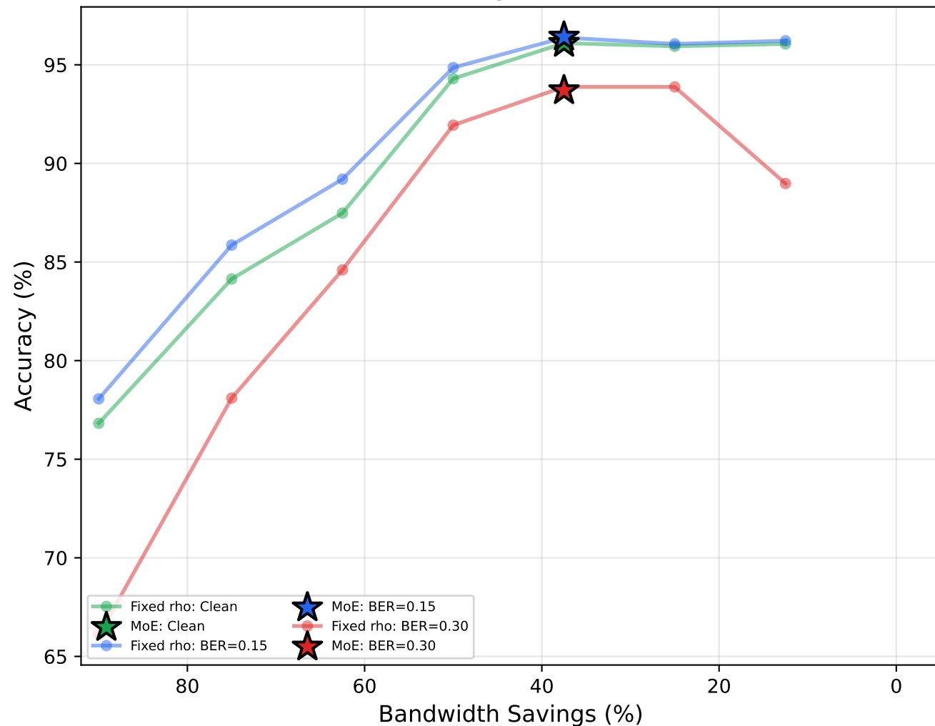
AID: Rate-Accuracy with Adaptive MoE (MoE stars = expert-selected rho)
