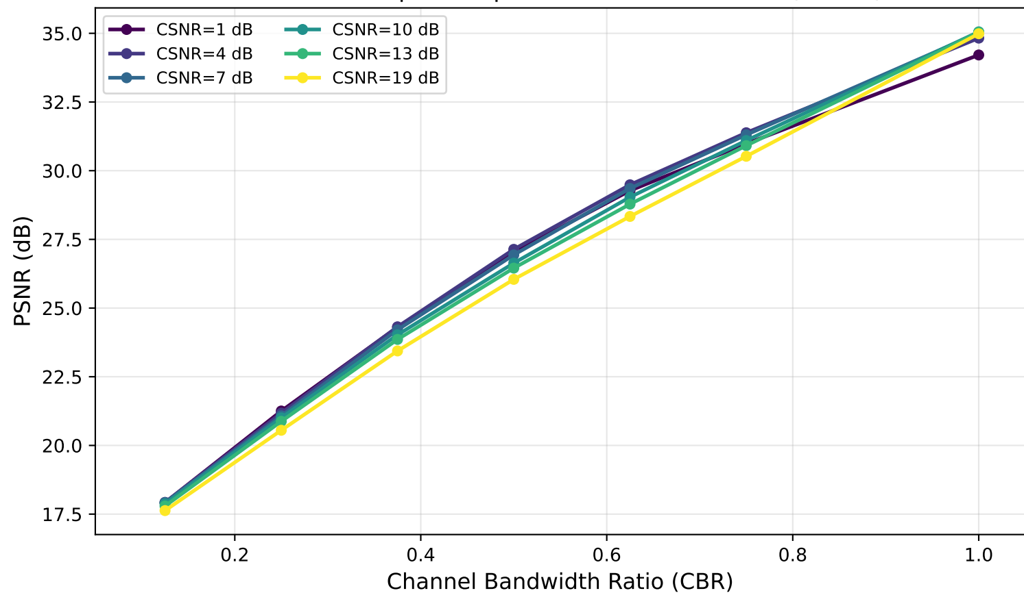
InStereo2K: SpikeAdapt-SC V6 Reconstruction (AWGN)
