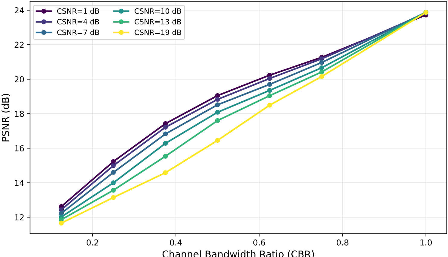
KITTI: SpikeAdapt-SC V6 Reconstruction (AWGN)
