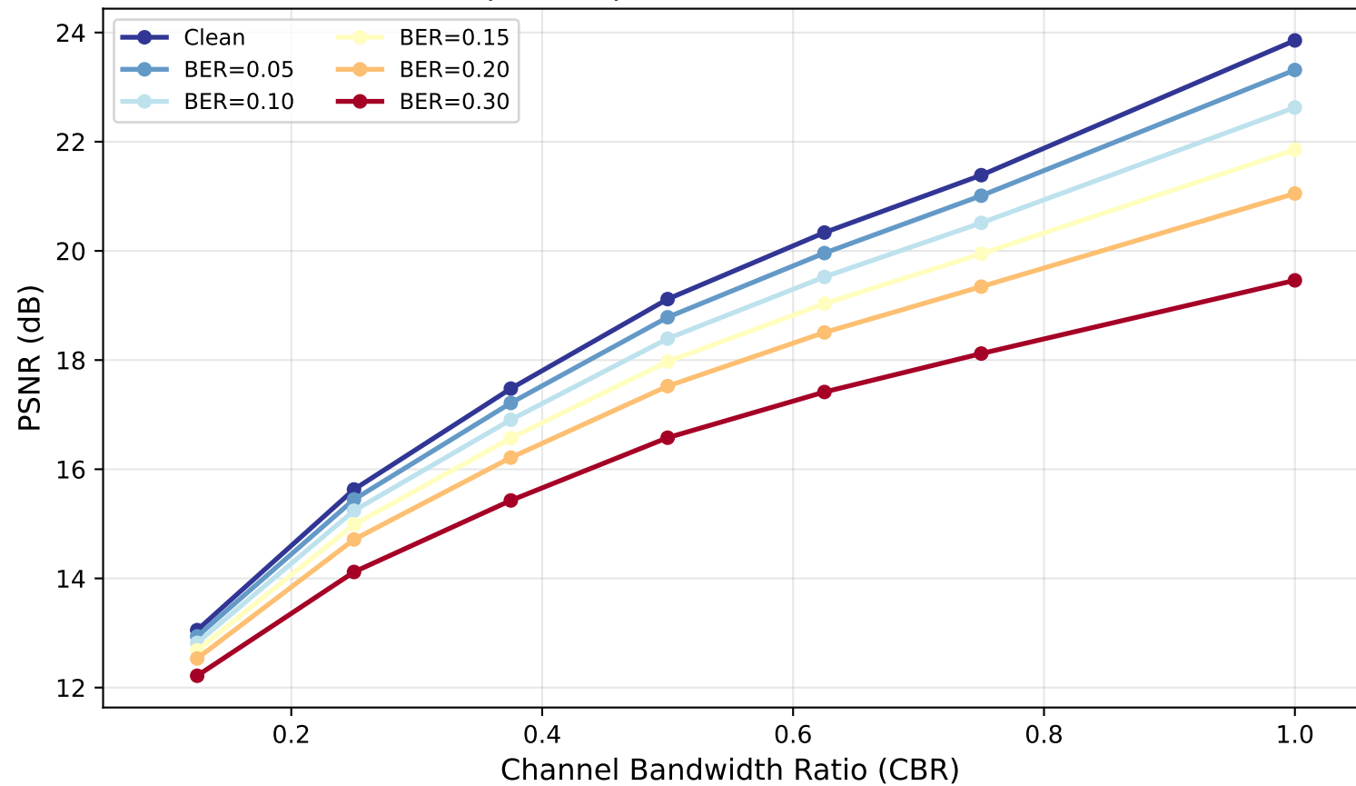
KITTI: SpikeAdapt-SC V6 Reconstruction (BSC)
