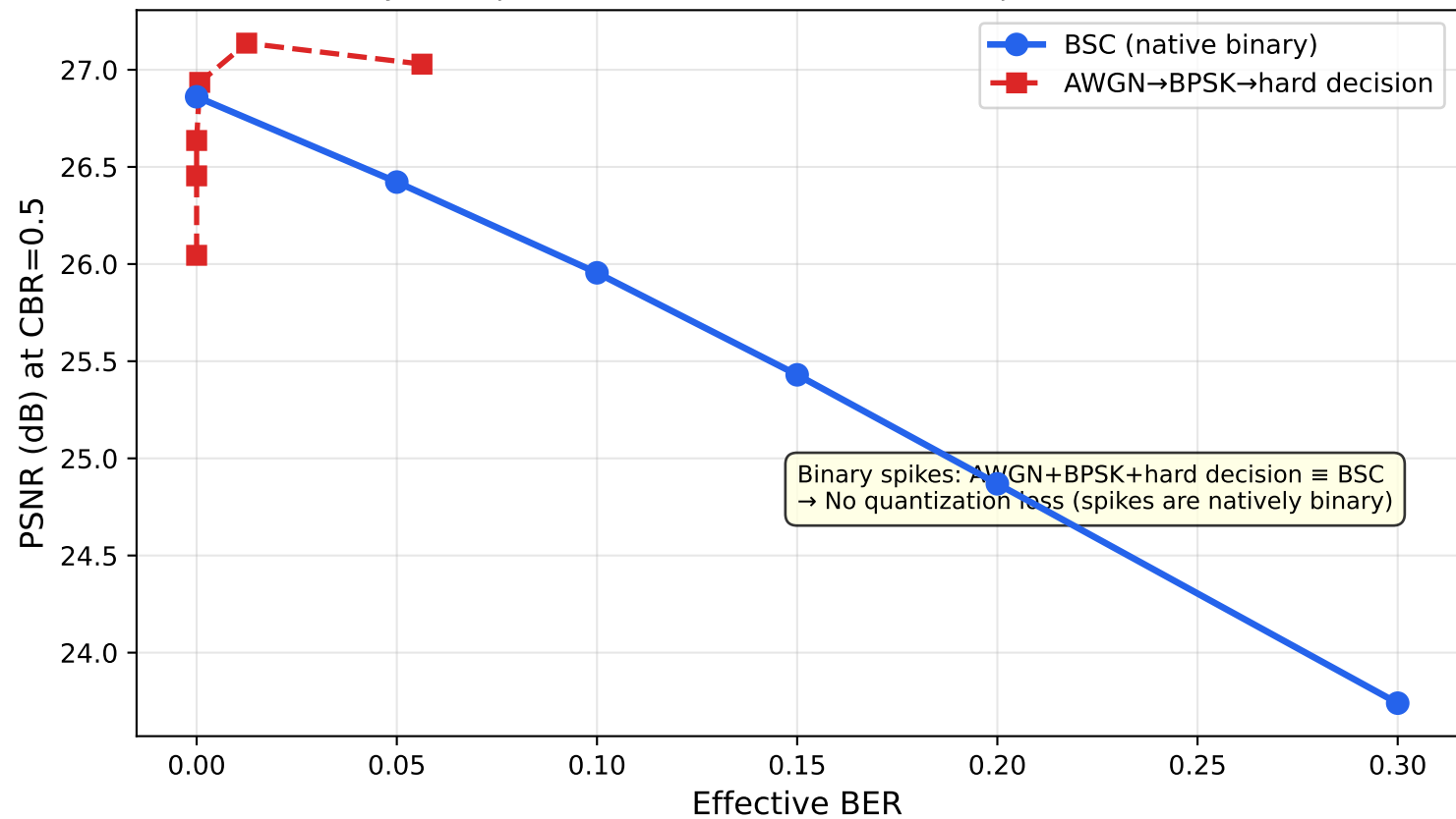
InStereo2K: BSC vs AWGN at Matched BER (CBR=0.5) Binary SNN spikes see identical channels \rightarrow no quantization needed
