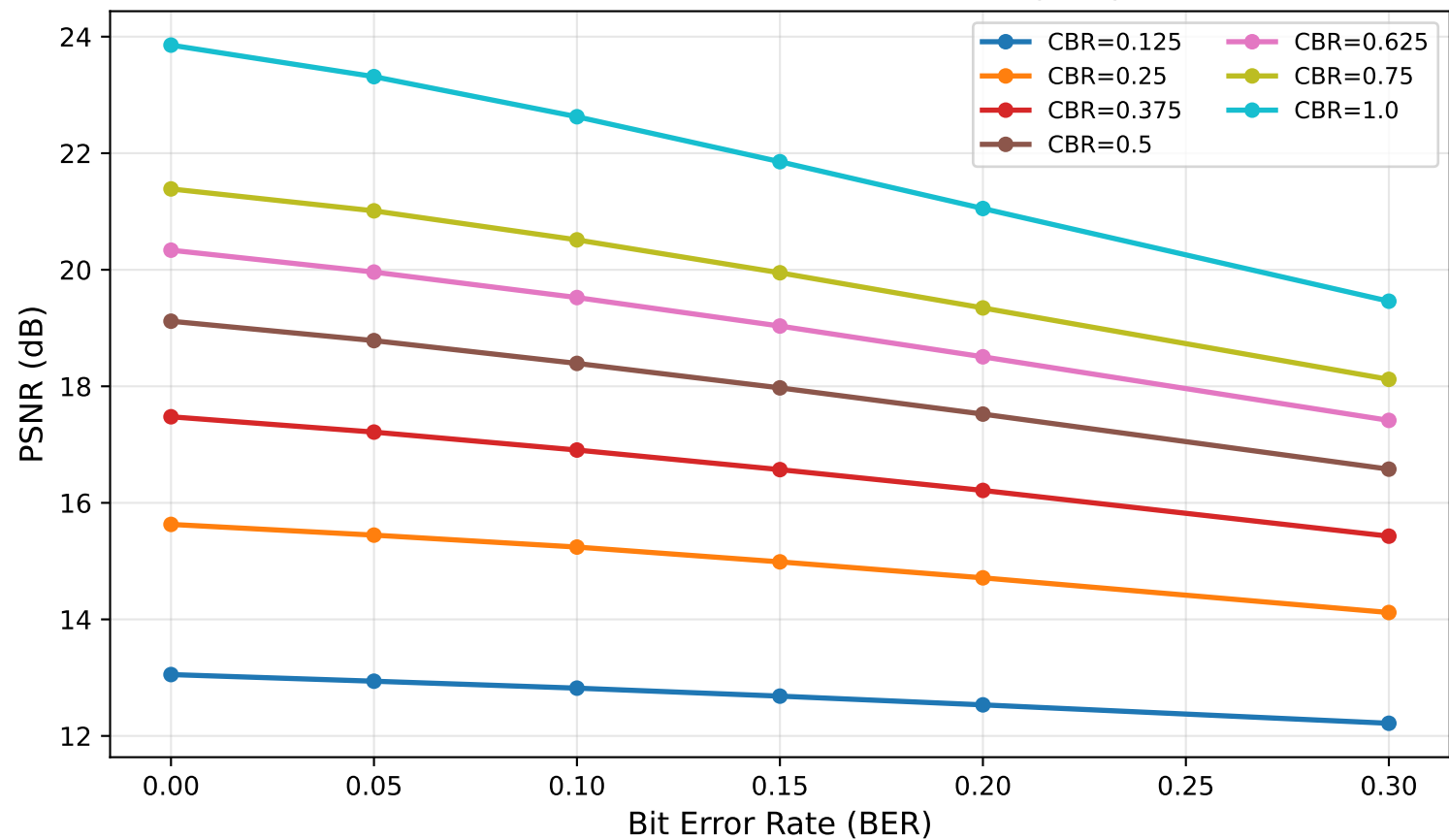
KITTI: Reconstruction PSNR vs BER (BSC)
