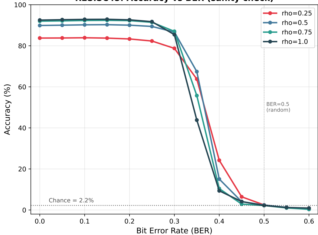
RESISC45: Accuracy vs BER (sanity check)
