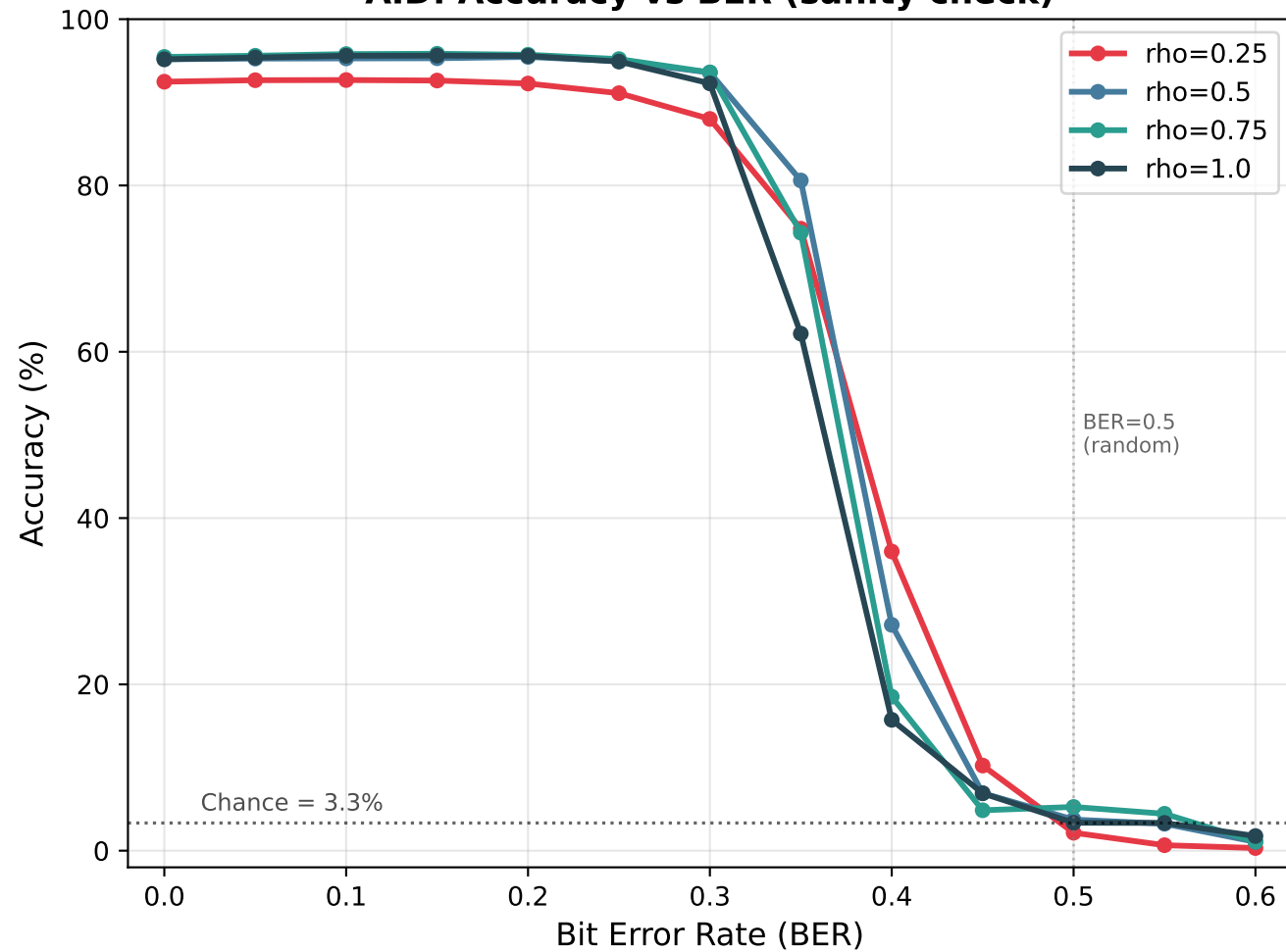
AID: Accuracy vs BER (sanity check)
