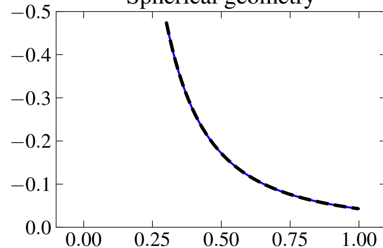
Spherical geometry
