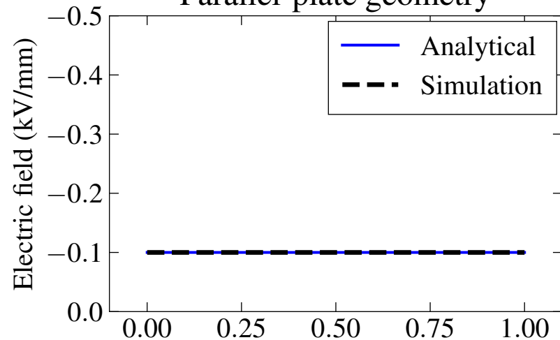
Parallel-plate geometry
