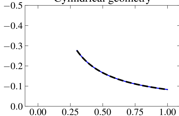
Cylindrical geometry
