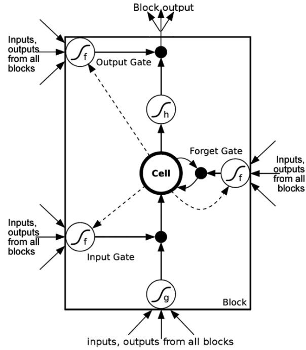
Figure 3: LSTM architecture
