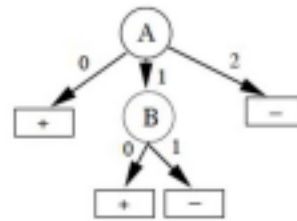
Figure 2: Pruned version of tree in Figure 1
