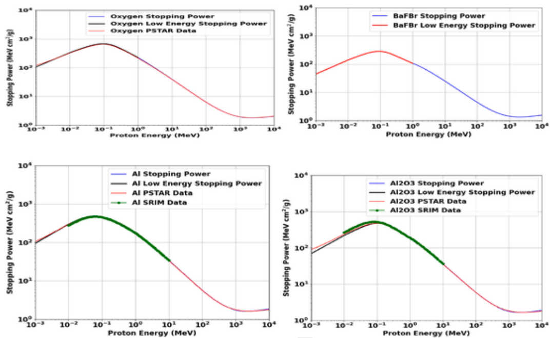
Fig. 2. Stopping power analysis for Oxygen, BaFBr, Aluminum, and Al_2O_3 across a broad proton energy range. Theoretical models (blue and black curves) align well with computed stopping powers from PSTAR (red curves) and SRIM-2008 (green markers). Minor deviations at lower energies for BaFBr suggest areas for model refinement. This analysis aids in material selection for dosimetry and understanding proton beam interactions.
