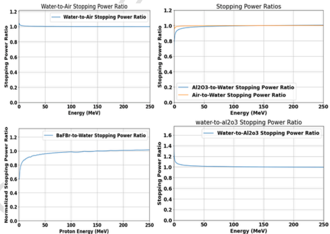
Fig. 3. Stopping power ratios for materials like water, air, Al_2O_3 , and BaFBr over the 0–250 MeV proton energy range. The water-to-air ratio remains stable, while the Al_2O_3 -to-water and air-to-water ratios highlight their differing attenuation properties. The BaFBr-to-water ratio shows significant material-dependent differences, and the water-to- Al_2O_3 ratio is particularly relevant for proton therapy dosimetry calculations in medical physics. These ratios are crucial for normalizing dosimetry readings in proton therapy.
