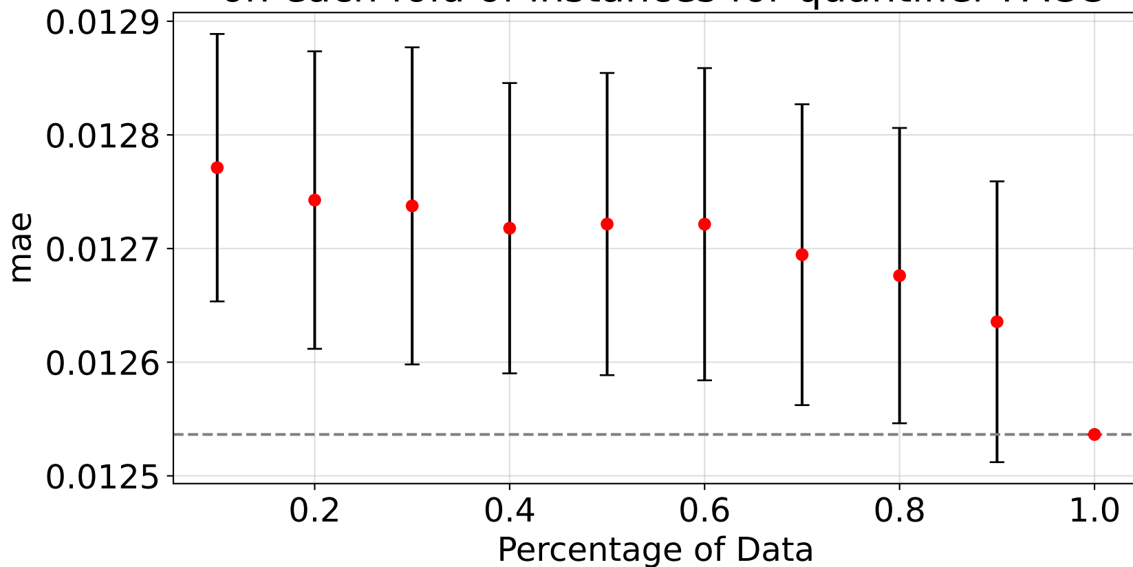
Additional Error of selecting other than the best configuration on each fold of instances for quantifier PACC
