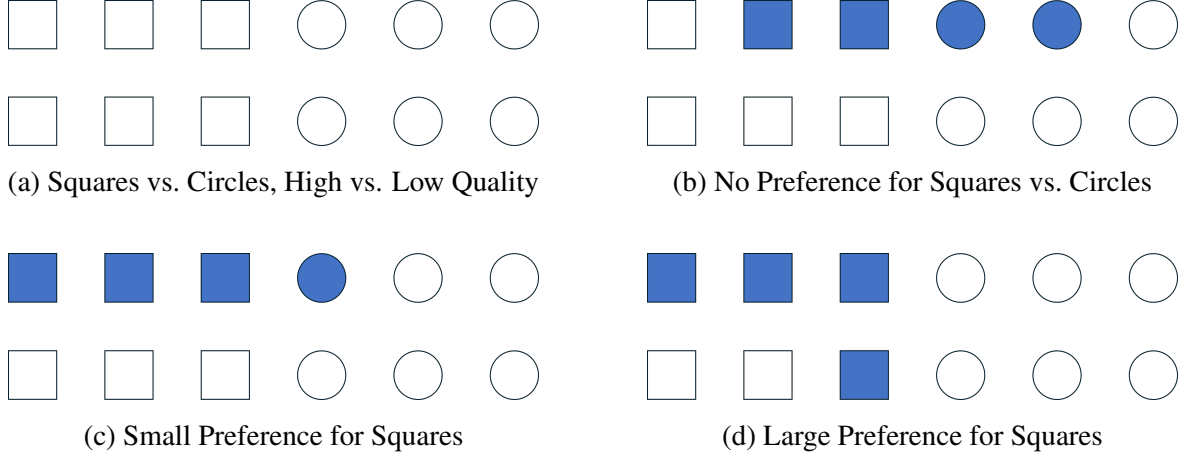
Figure 1: Diversity Objective
