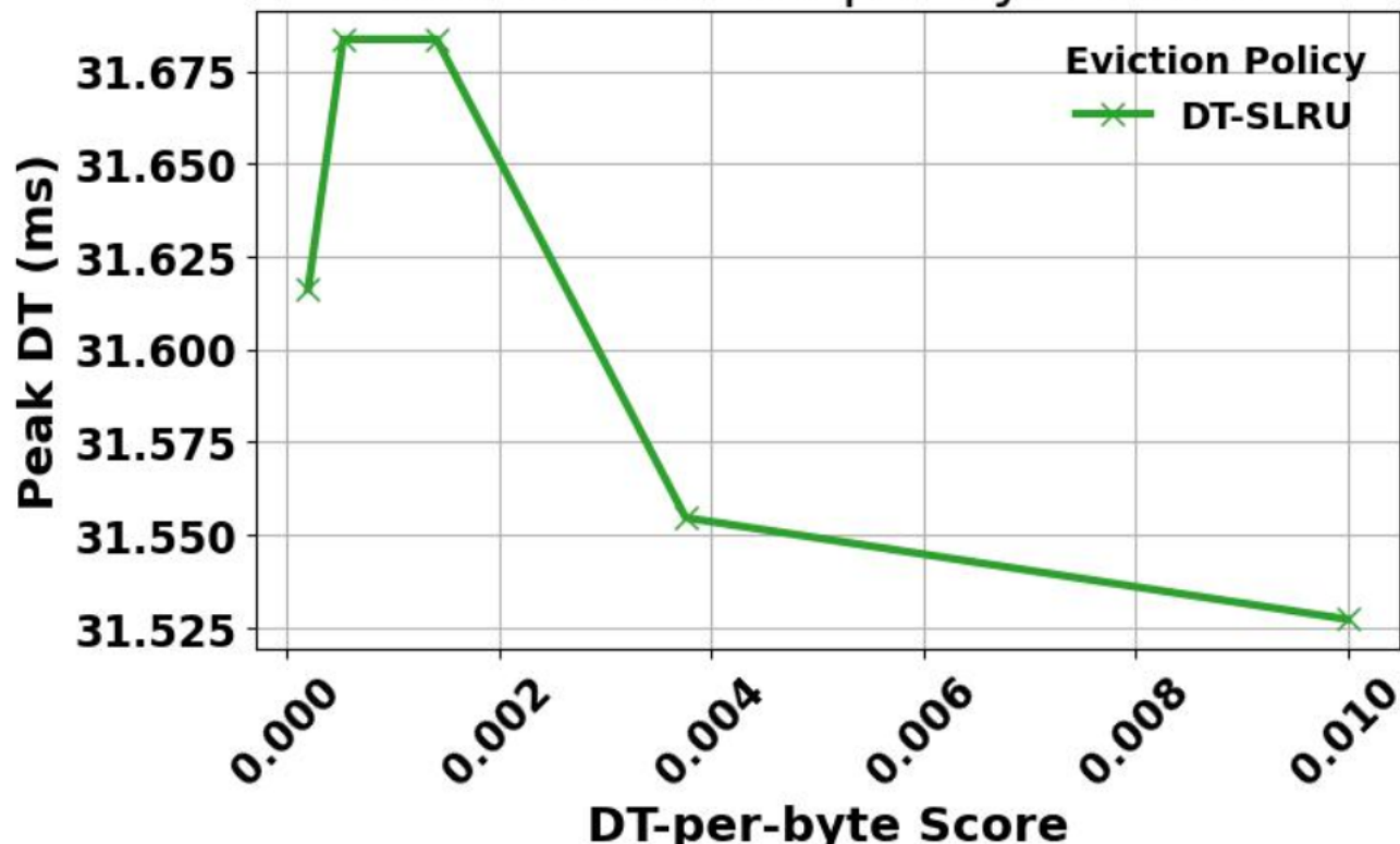
Peak DT vs. DT-per-byte Score
