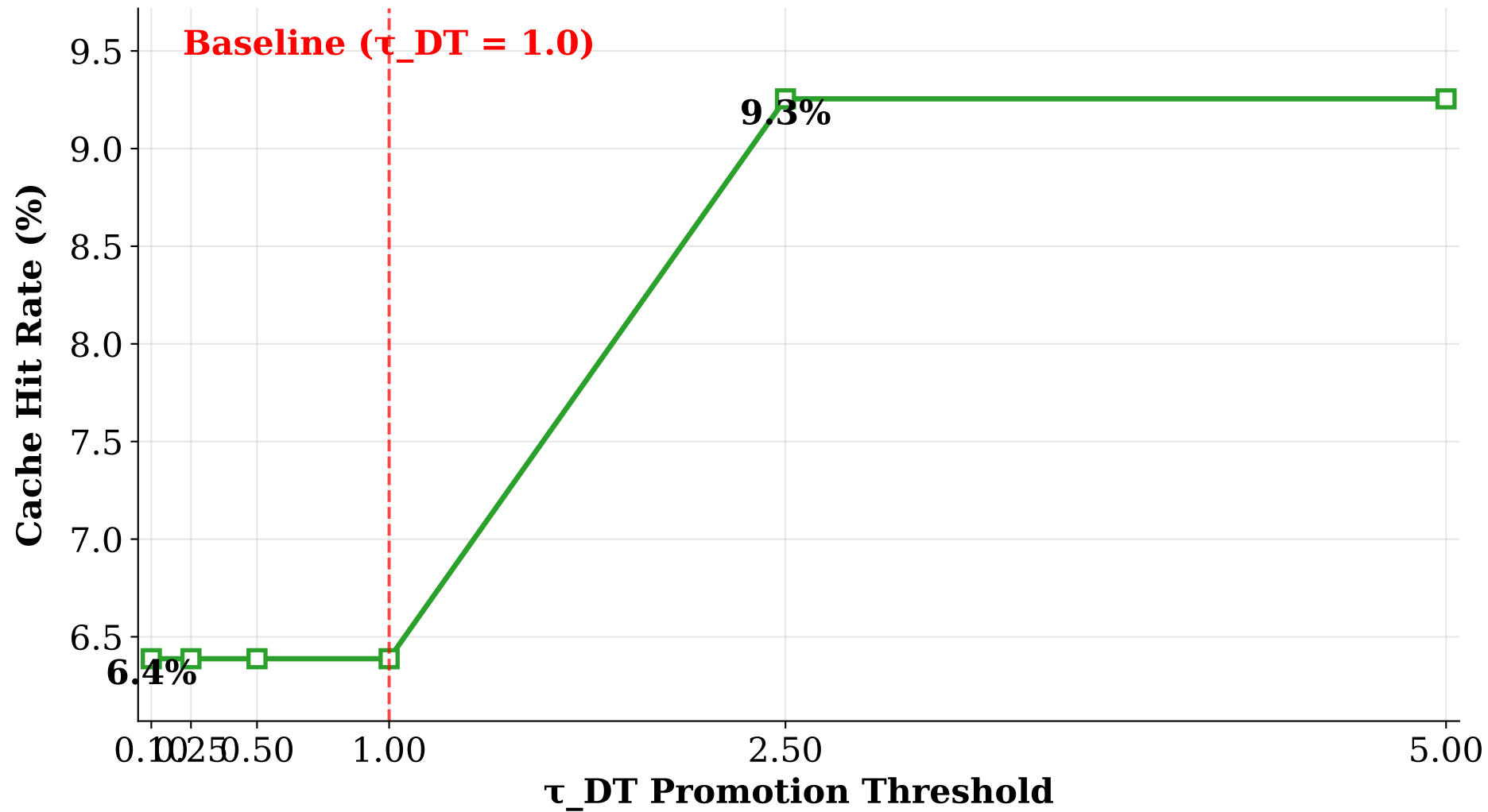
Figure 2: Hit Rate vs. \tau_{DT} (E1 DT-SLRU)
