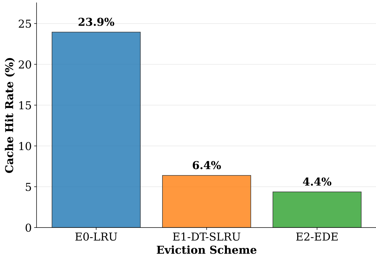
Figure 3: Cache Hit Rate (%) across eviction schemes (E0-E2)
