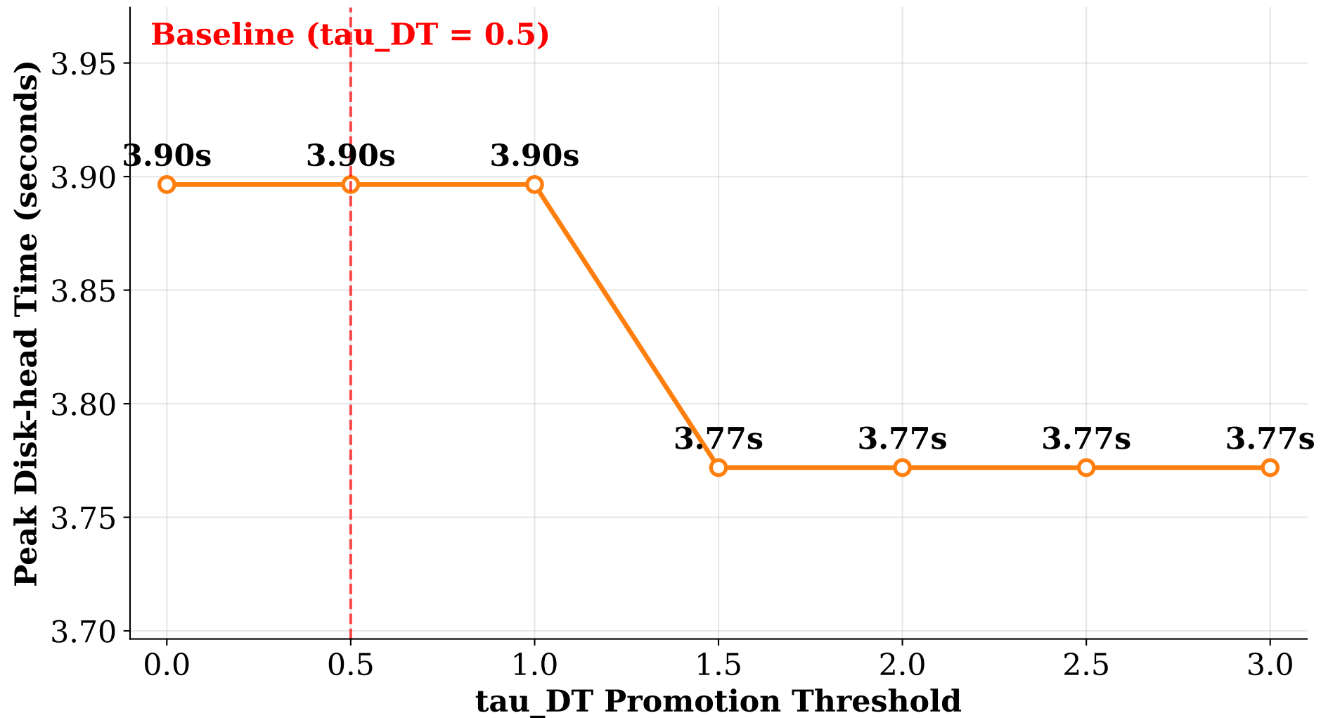
Figure 5: Peak DT vs. \tau_{DT} (E1 DT-SLRU)
