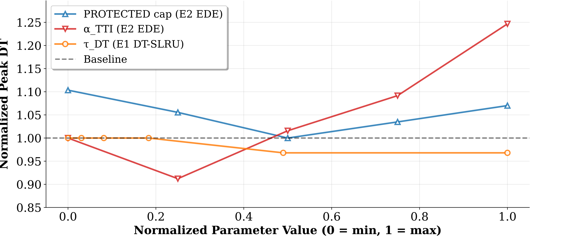
Figure 5: Combined Sensitivity Summary: Normalized Peak DT for All Ablated Parameters
