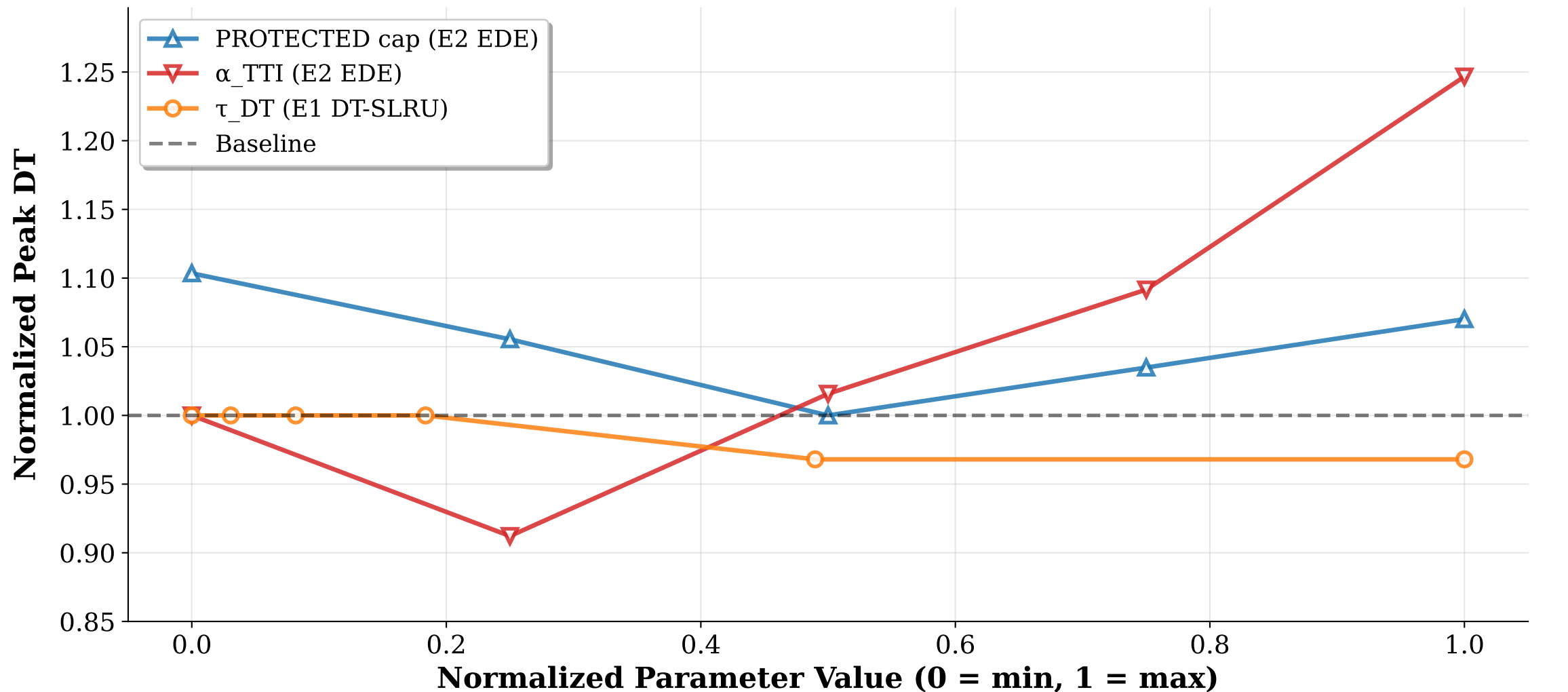
Figure 5: Combined Sensitivity Summary: Normalized Peak DT for All Ablated Parameters
