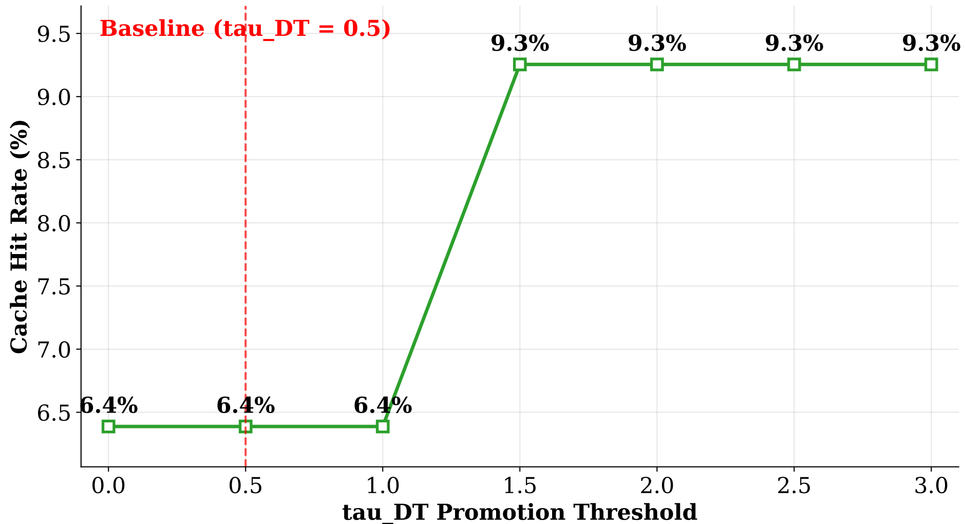
Figure 5: Hit Rate vs. \tau_{DT} (E1 DT-SLRU)
