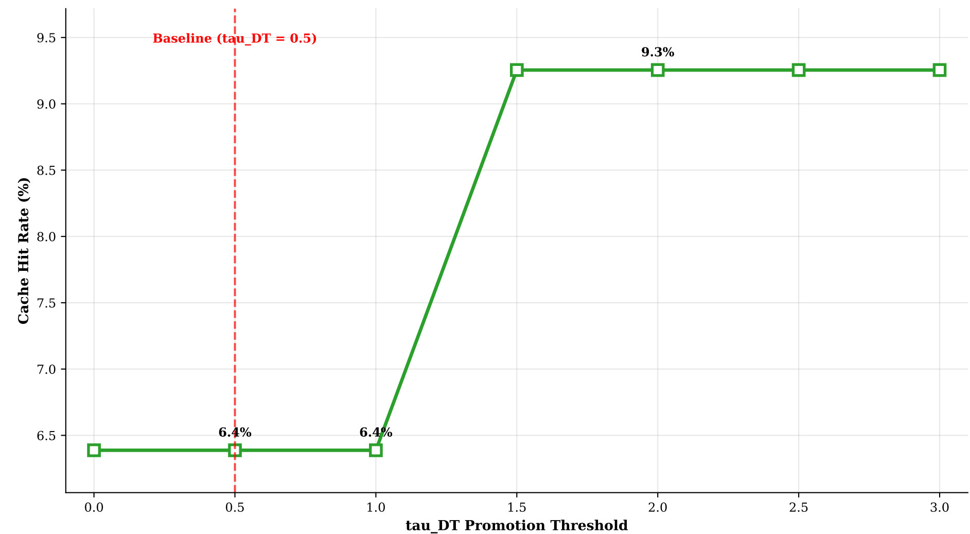
(b) Hit Rate vs. tau_DT (Context)
