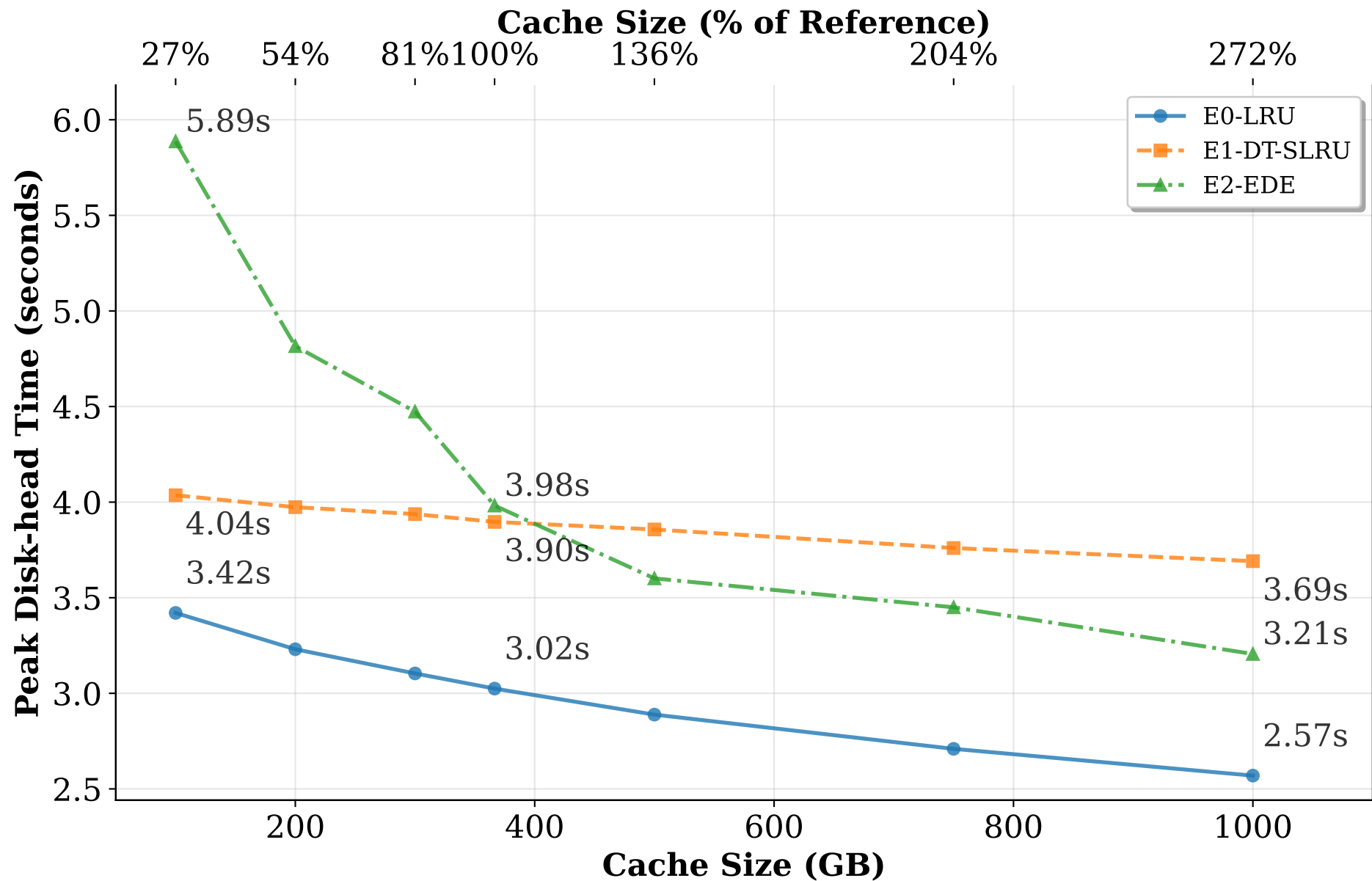
Figure 4: Peak DT vs. Cache Size (E0-E2 comparison)
