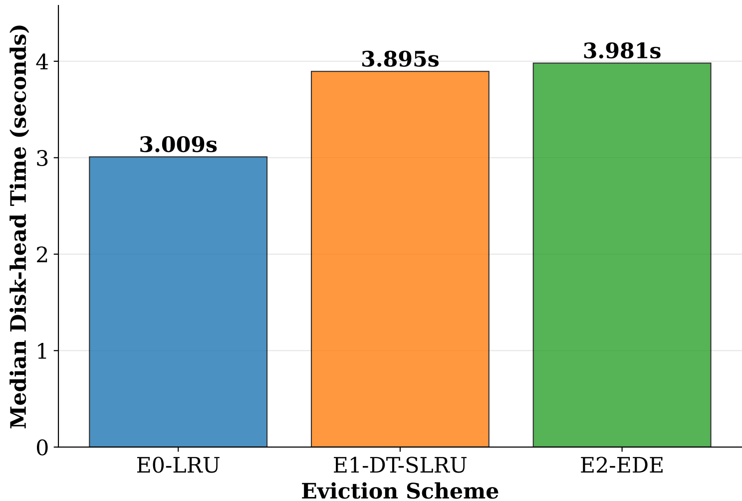
Figure 2: Median DT across eviction schemes (E0-E2)
