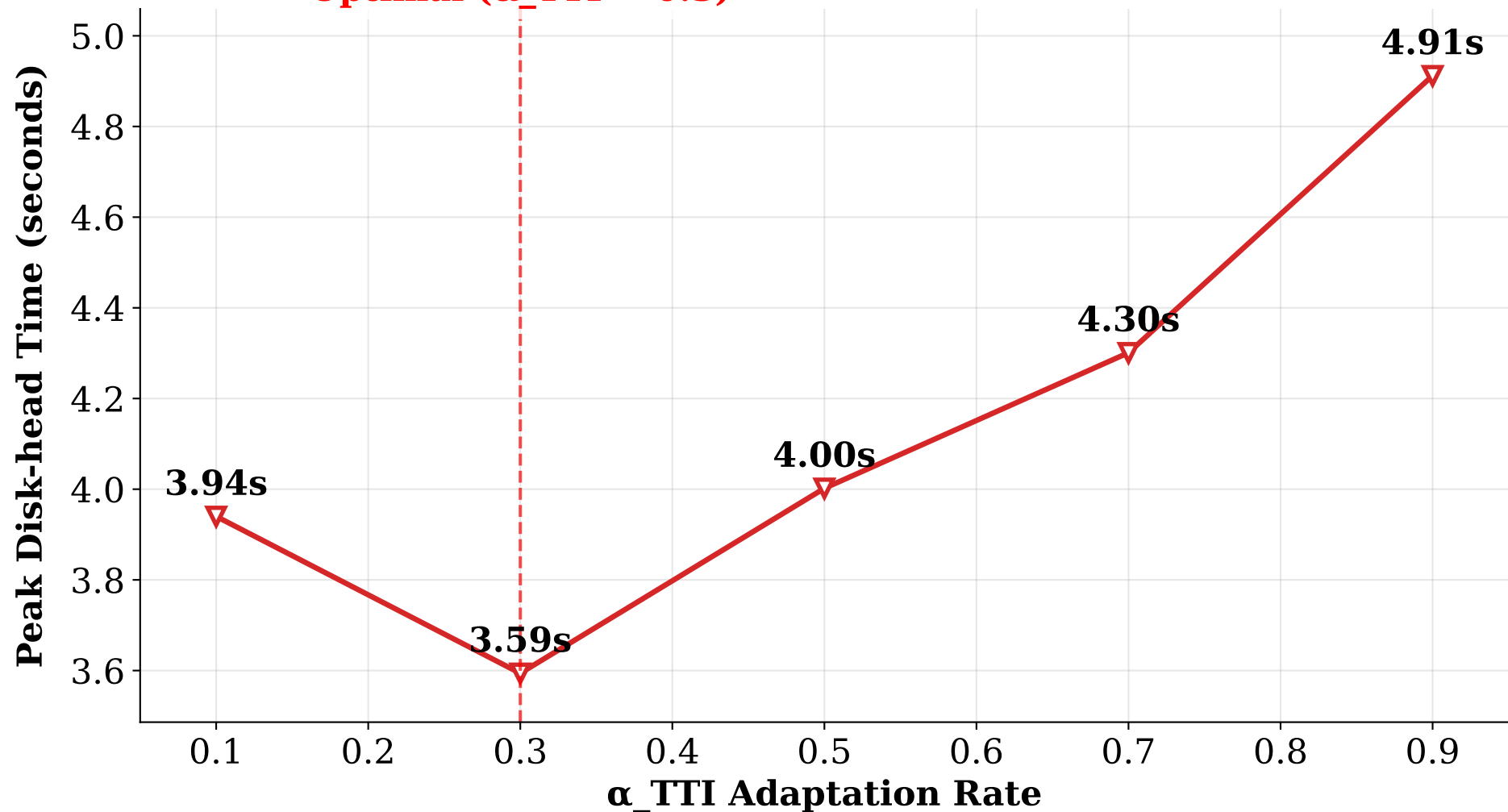
Figure 4: Peak DT vs. \alpha_{TTI} (E2 EDE) Optimal ( \alpha_{TTI} = 0.3 )
