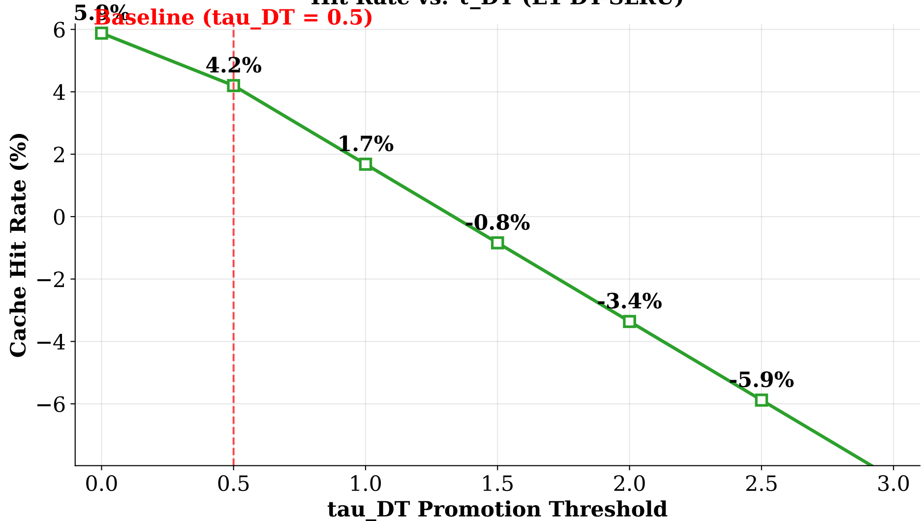
Hit Rate vs. \tau_{DT} (E1 DT-SLRU)
