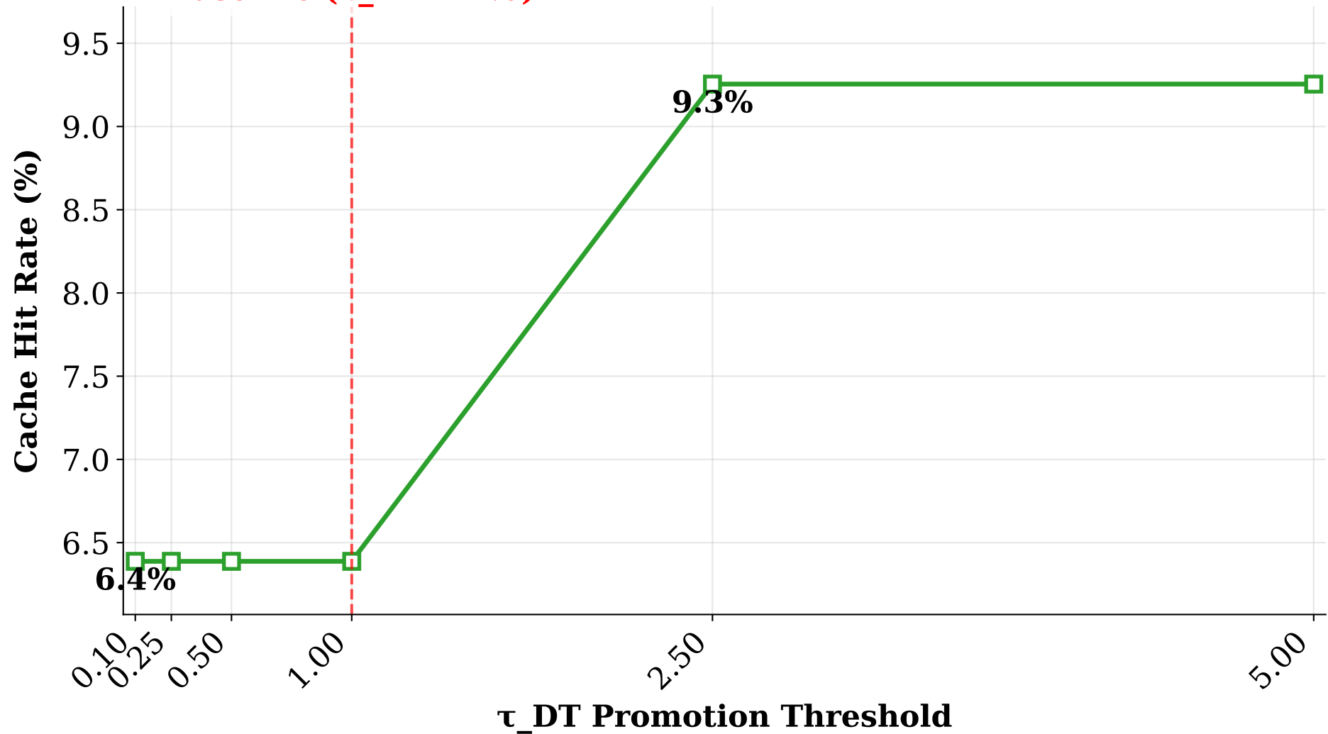
Hit Rate vs. \tau_{DT} (E1 DT-SLRU)
