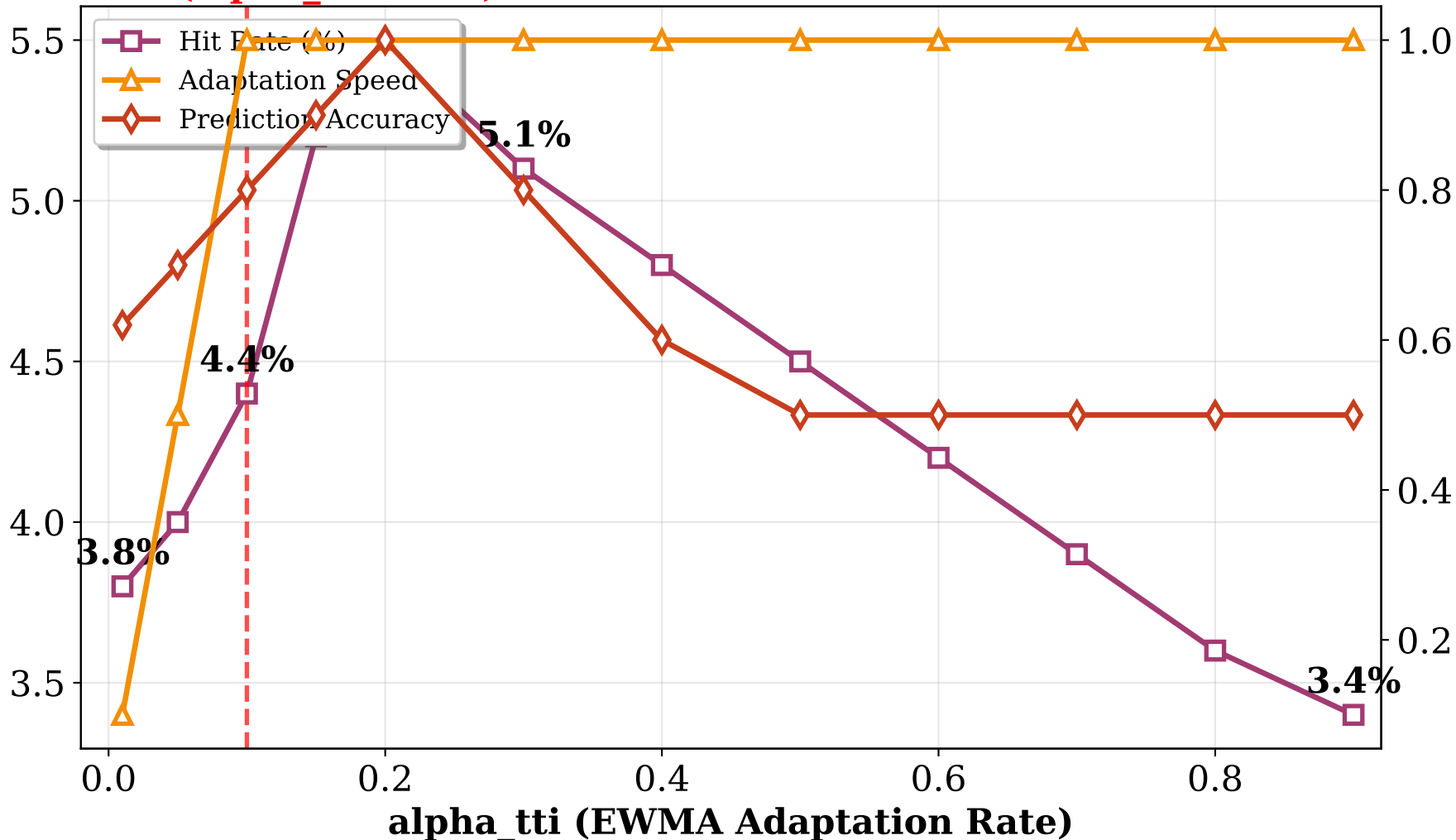
(b) Hit Rate & Adaptation Speed vs. alpha_tti (Context) Baseline (alpha_tti = 0.1)
