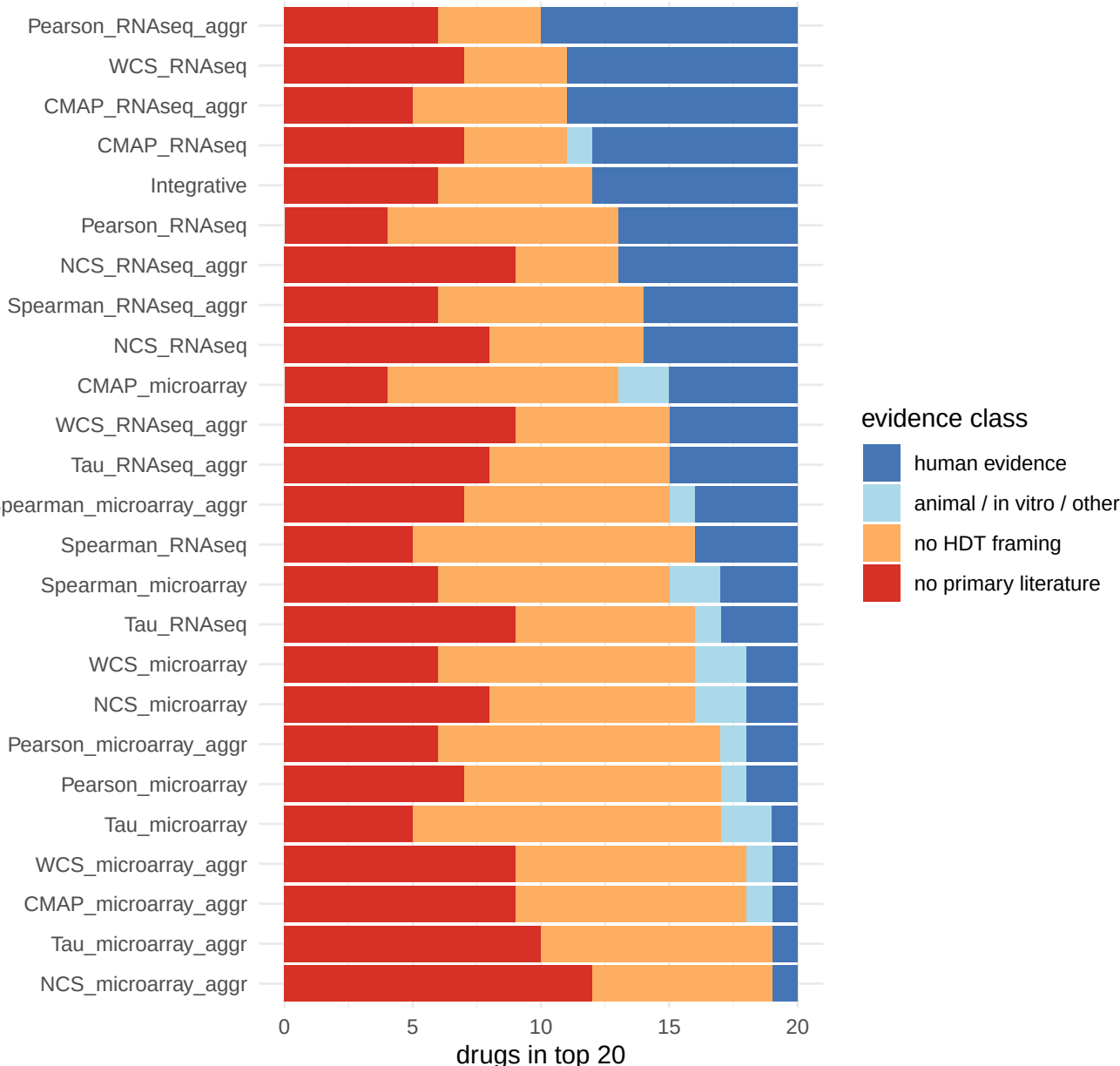
Evidence supporting the top 20 predictions of each method strongest evidence available per drug, sorted by drugs with human evidence
