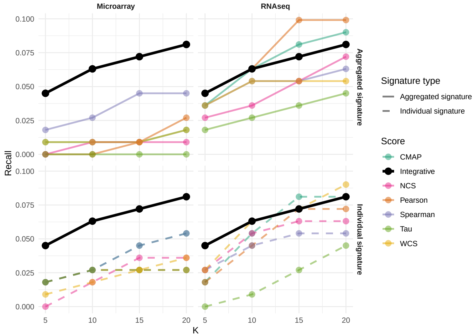
Recall@K across methods by technology and signature type
