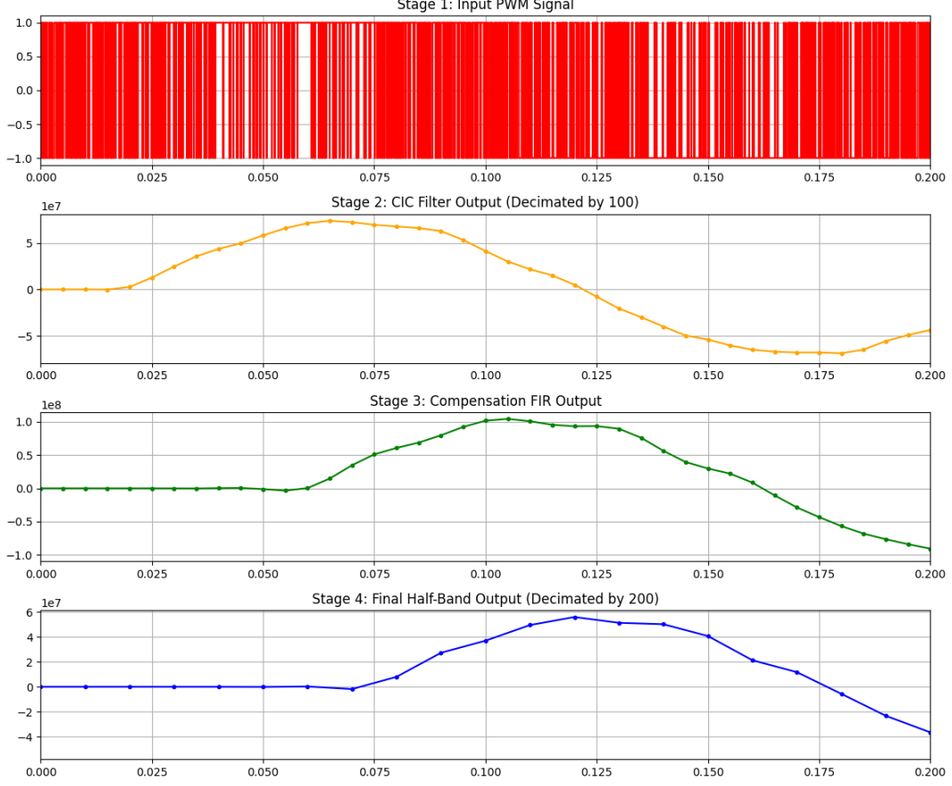
Figure 9: Time-Domain Output of Decimation Stages for f = 20\text{Hz} (High Noise Environment)
