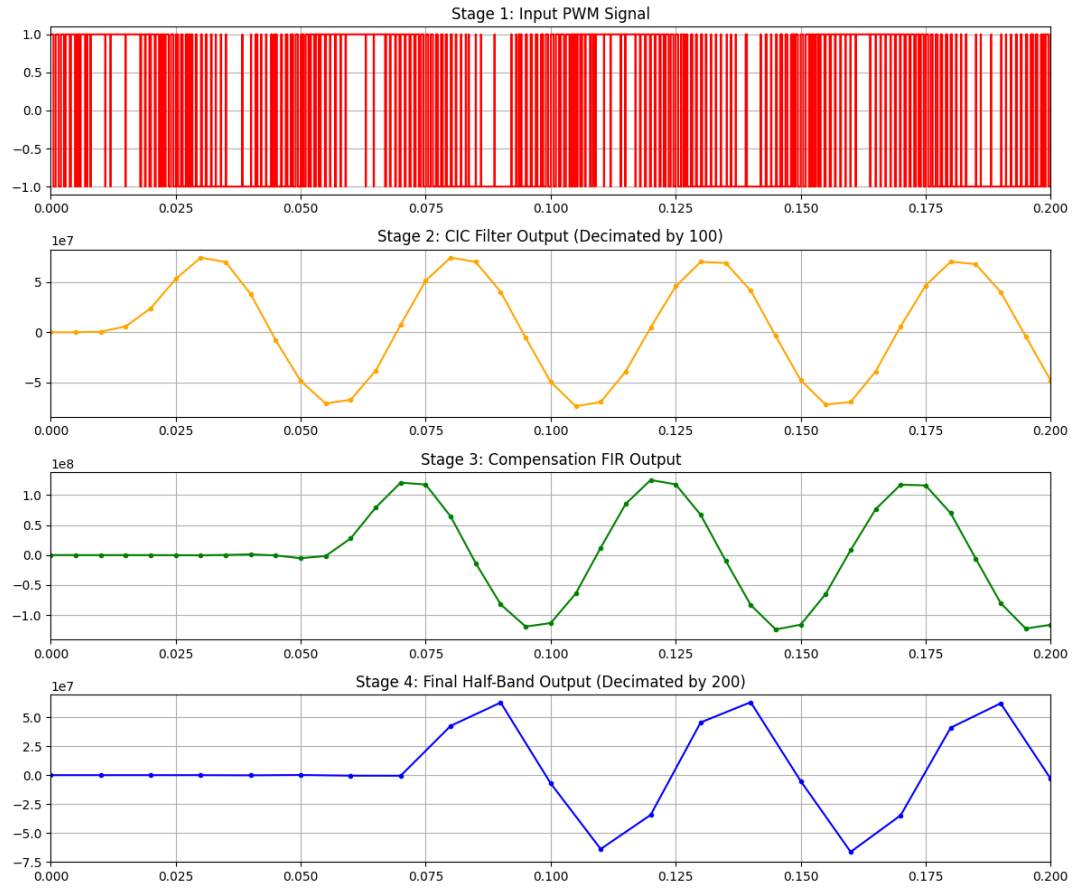
Figure 6: Time-Domain Output of Decimation Stages for f = 20\text{Hz}
