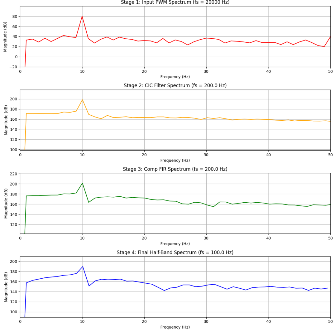
Figure 7: Frequency Spectra Across the Decimation Chain
