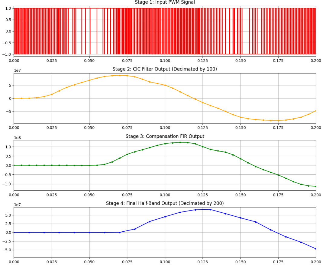
Figure 8: Time-Domain Details Demonstrating Filter Smoothing under Moderate Noise
