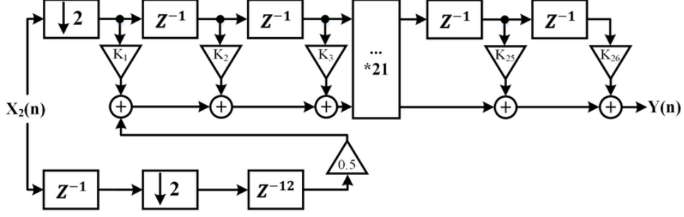
Figure 5: Structure of the Multiphase Half-Band Filter
