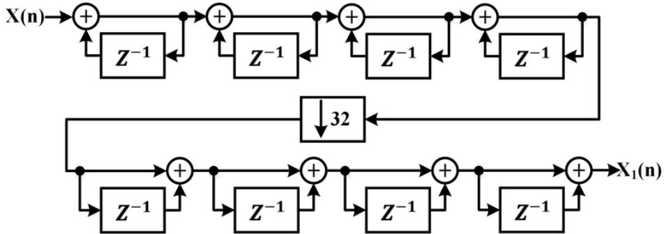
Figure 3: Structure of the CIC Decimation Filter
