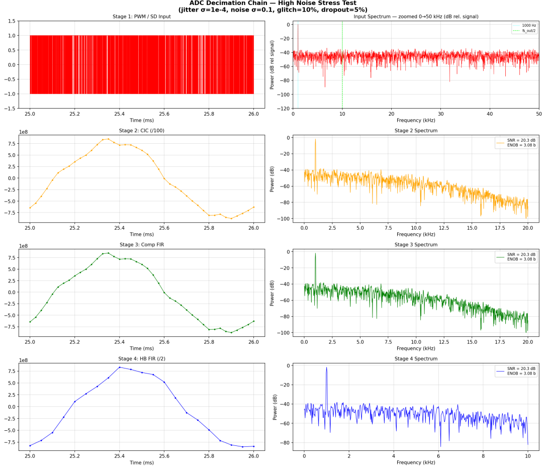
Figure 9: Single-Cycle Time-Domain and Spectral Output under High-Noise Stress ( f_{sig} = 1 \text{ kHz} )
