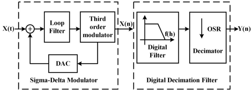
Figure 1: General Block Diagram of a Sigma-Delta ADC
