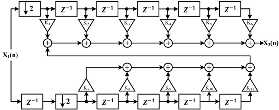
Figure 4: Structure of the Multiphase Compensation Filter
