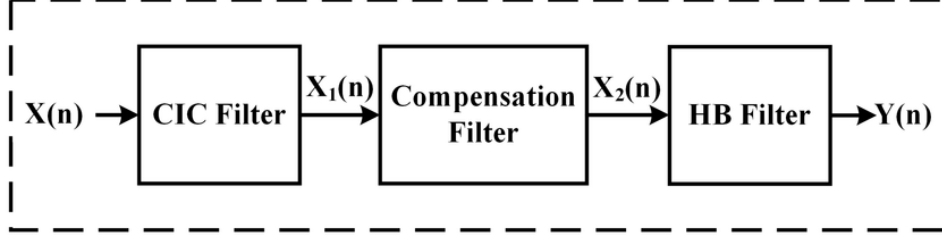
Figure 2: Block Diagram of the Three-Stage Digital Decimation Filter
