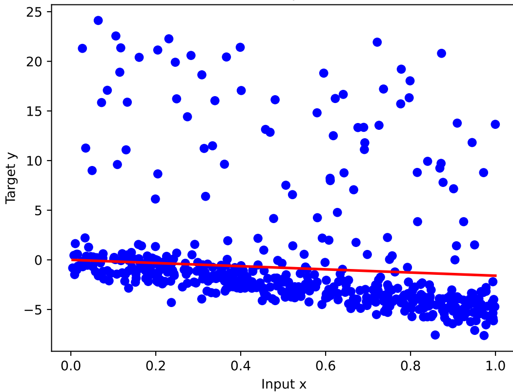
Least Squares
