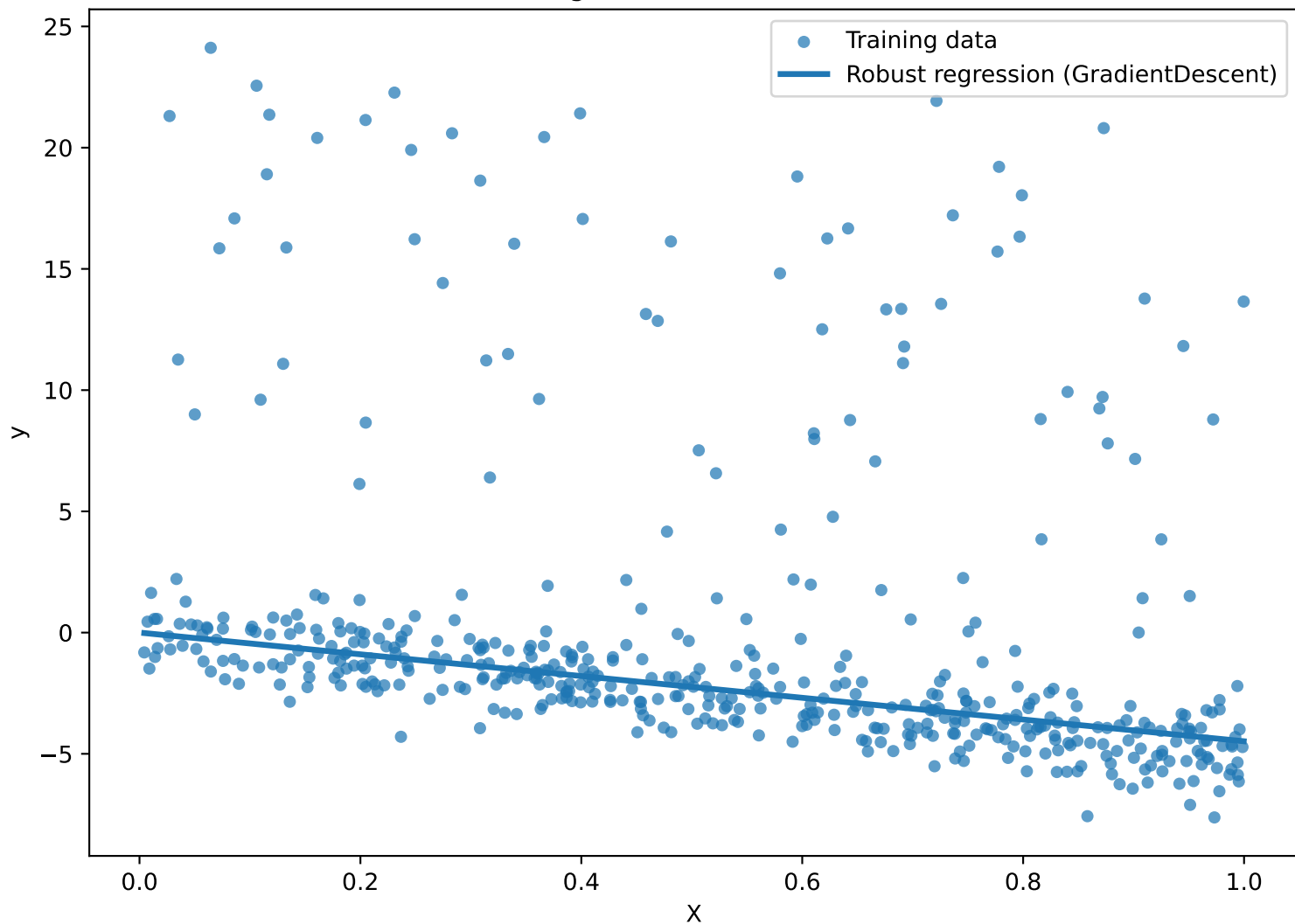
Robust Regression - Gradient Descent
