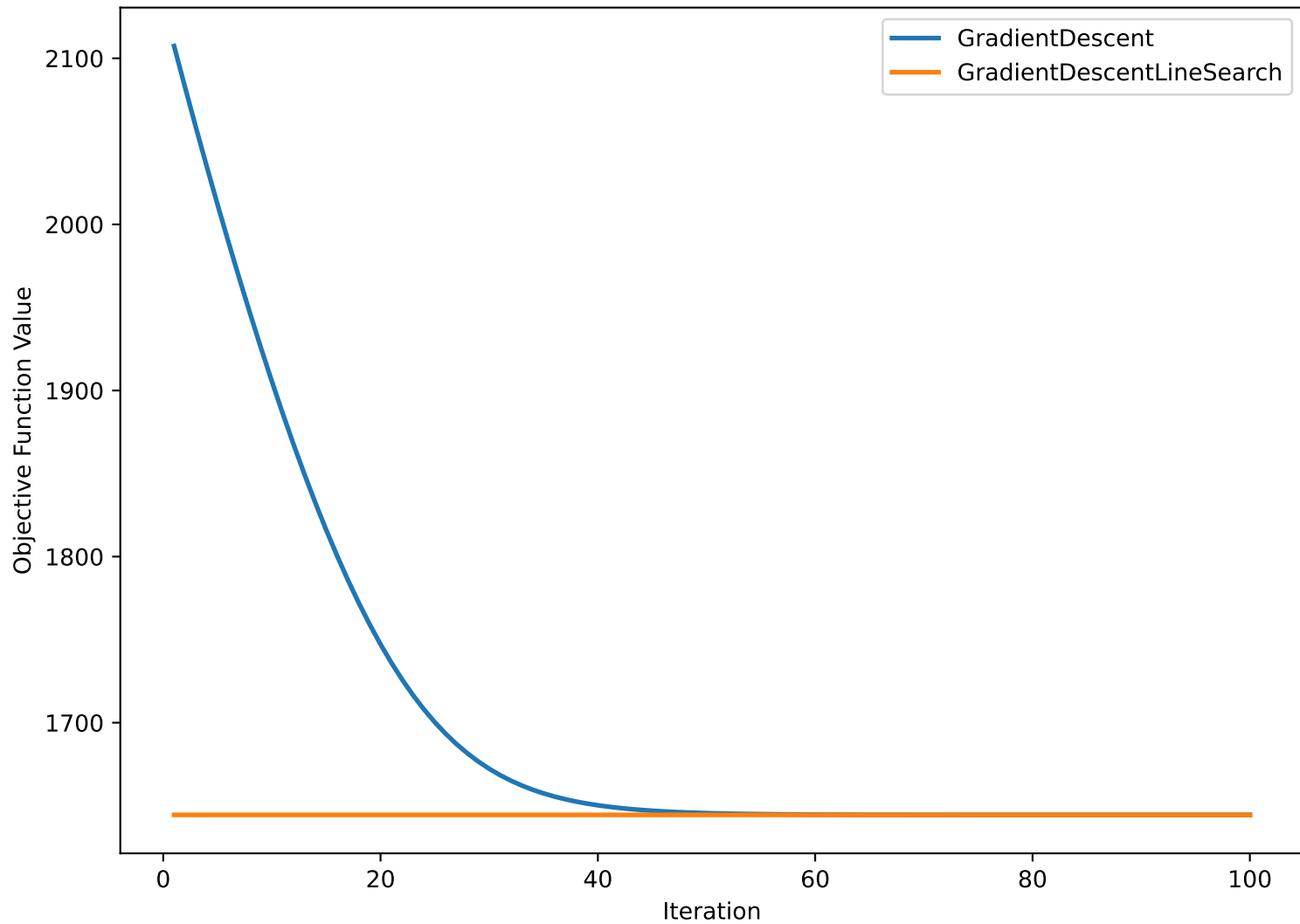
Robust Regression: Optimizer Comparison
