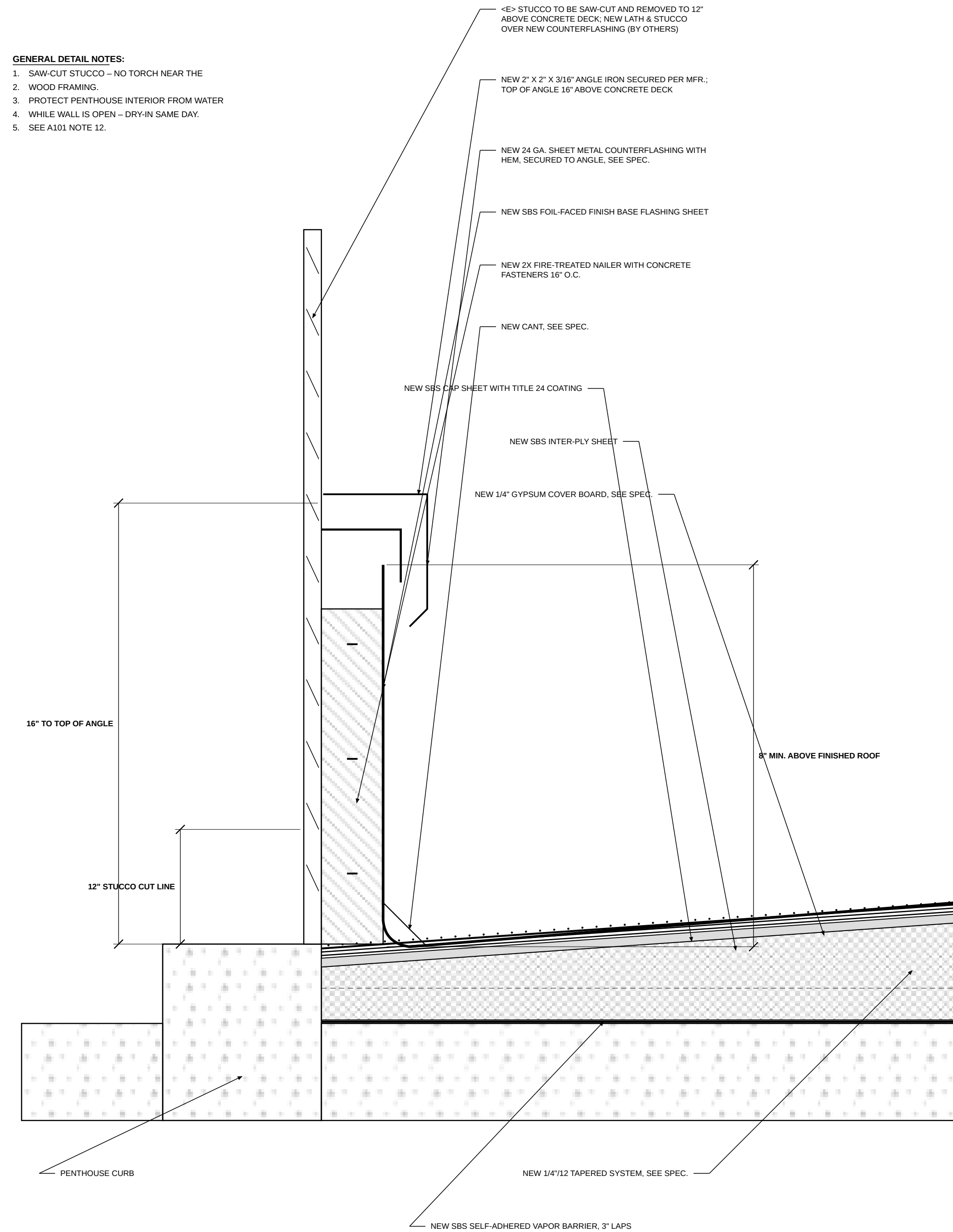
1 PENTHOUSE WALL DETAIL
