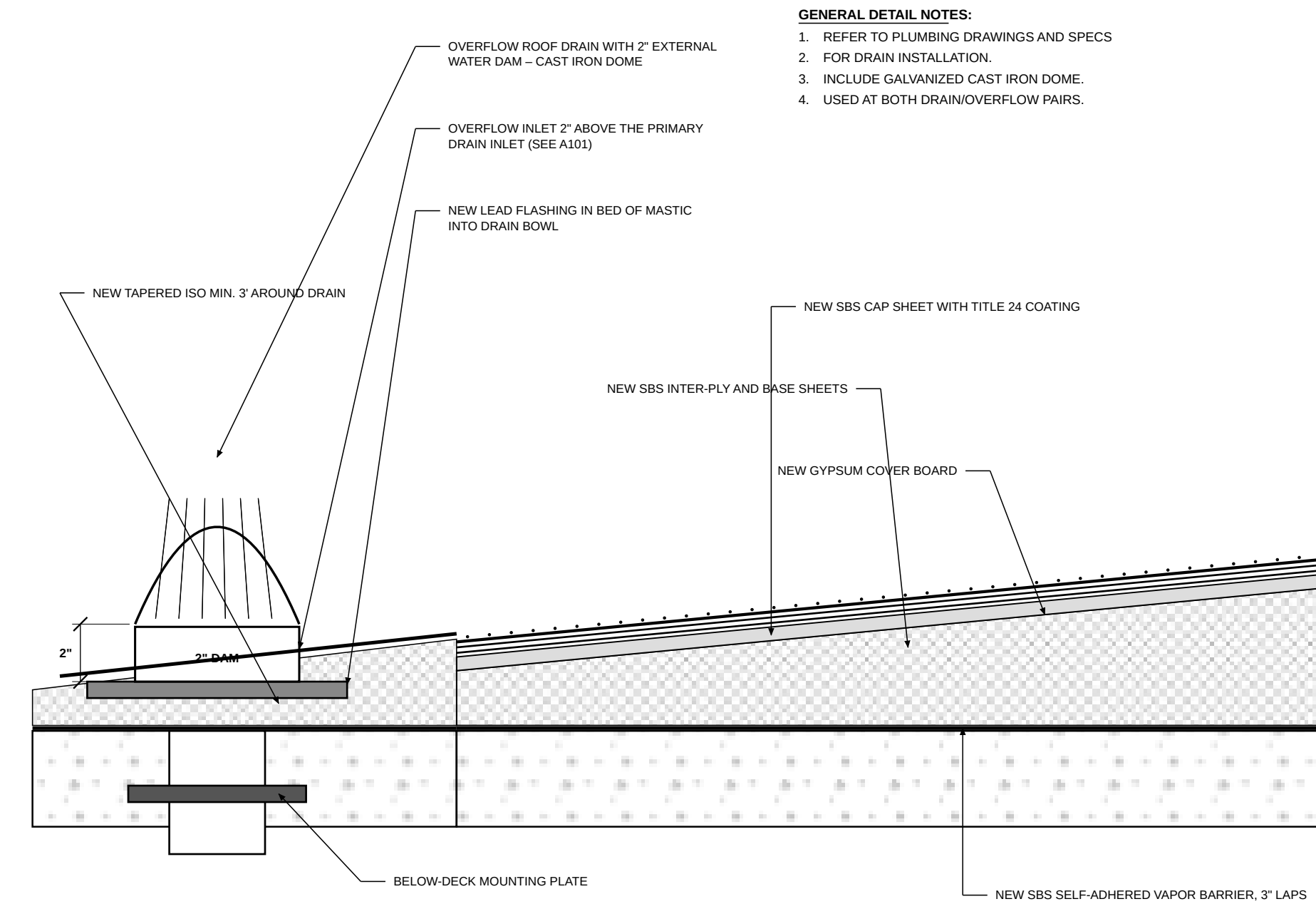
6 ROOF DRAIN OVERFLOW
