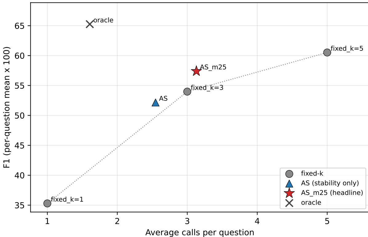
Distractor cells: macro across 3 models x {HotpotQA, 2Wiki}
