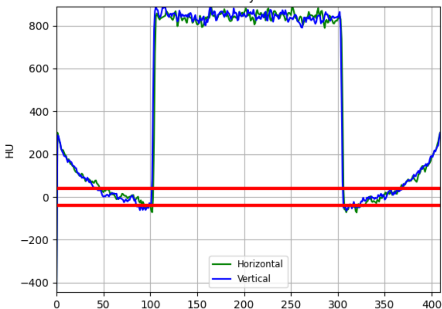
Uniformity Profiles
