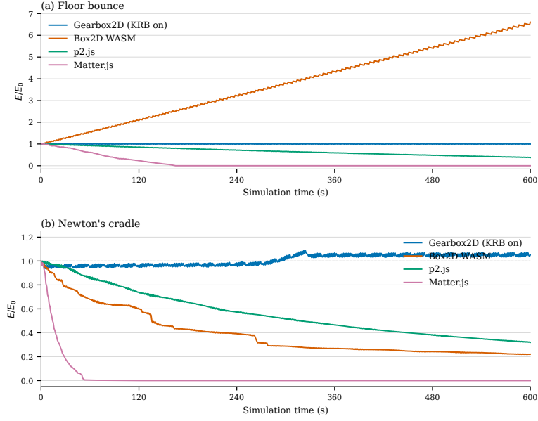
Figure 3. Mechanical energy ratio E/E_0 over 600 s. Gearbox2D is a native KRB-on recapture (translational meter); Box2D-WASM, p2.js, and Matter.js are unmodified website exports. (a) Elastic floor contact. (b) Newton's cradle.
