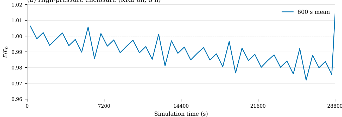
(b) High-pressure enclosure (KRB on, 8 h)
