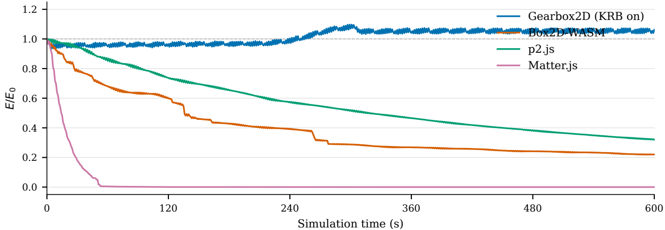
(b) Newton's cradle
