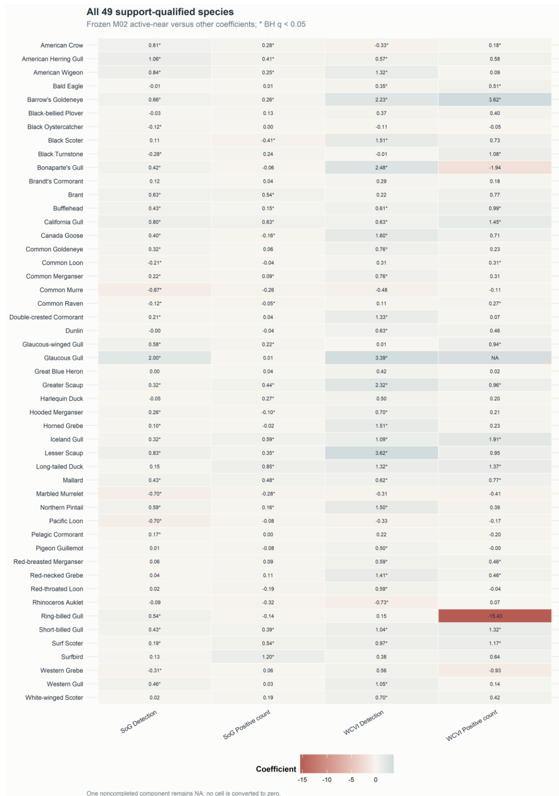
Figure S3. Complete 49-species coefficient matrix. Values are frozen M02 coefficients for active-near versus other. An asterisk indicates BH q < 0.05 . The noncompleted component remains NA.
