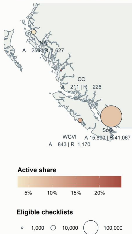
Figure S2. Region-level active and reference support. Display anchors are not data coordinates. All displayed regional cells exceed n = 20.
