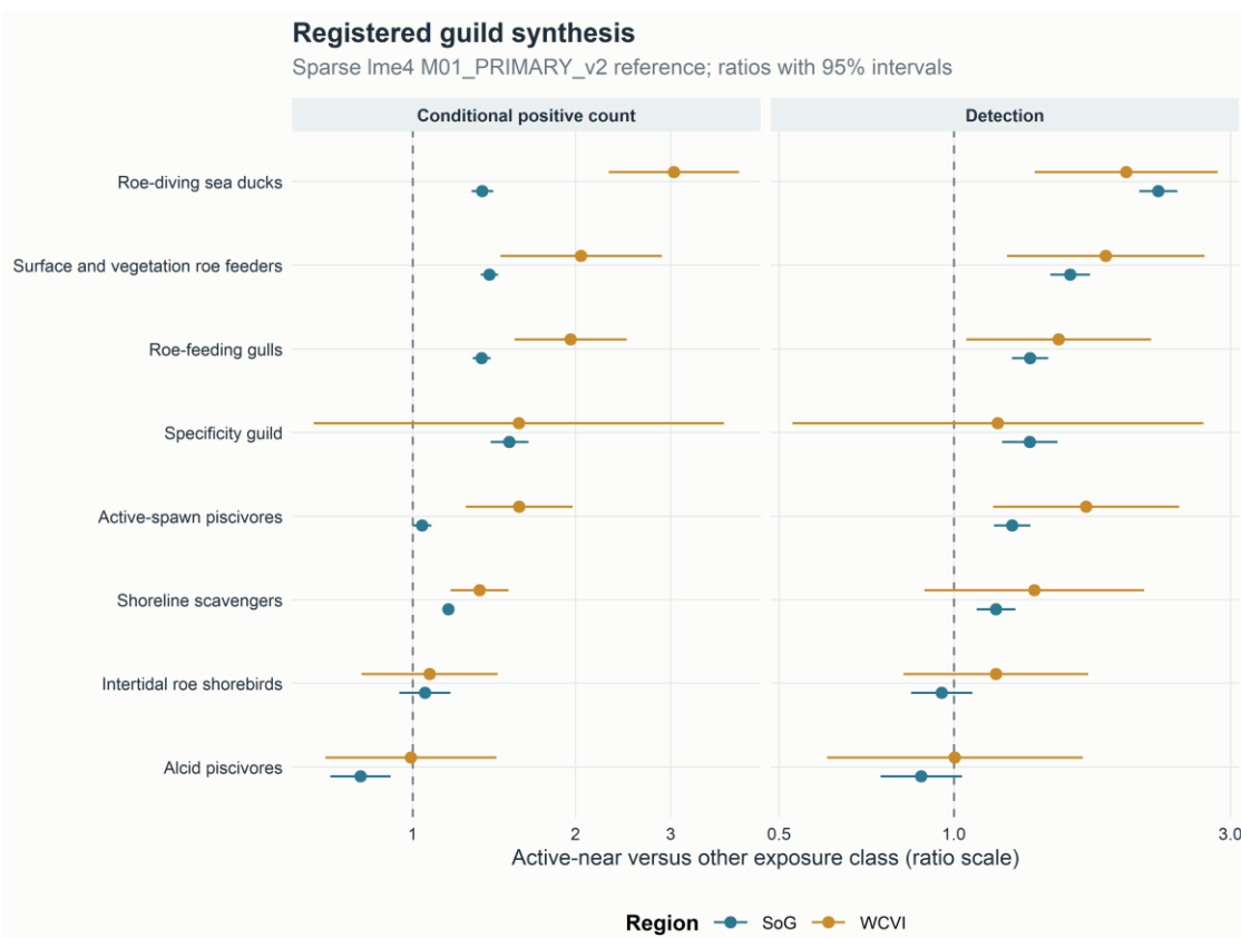
Figure S4. Sparse M01 guild synthesis. Ratios compare active-near with other. Guild averages complement rather than replace species evidence.
