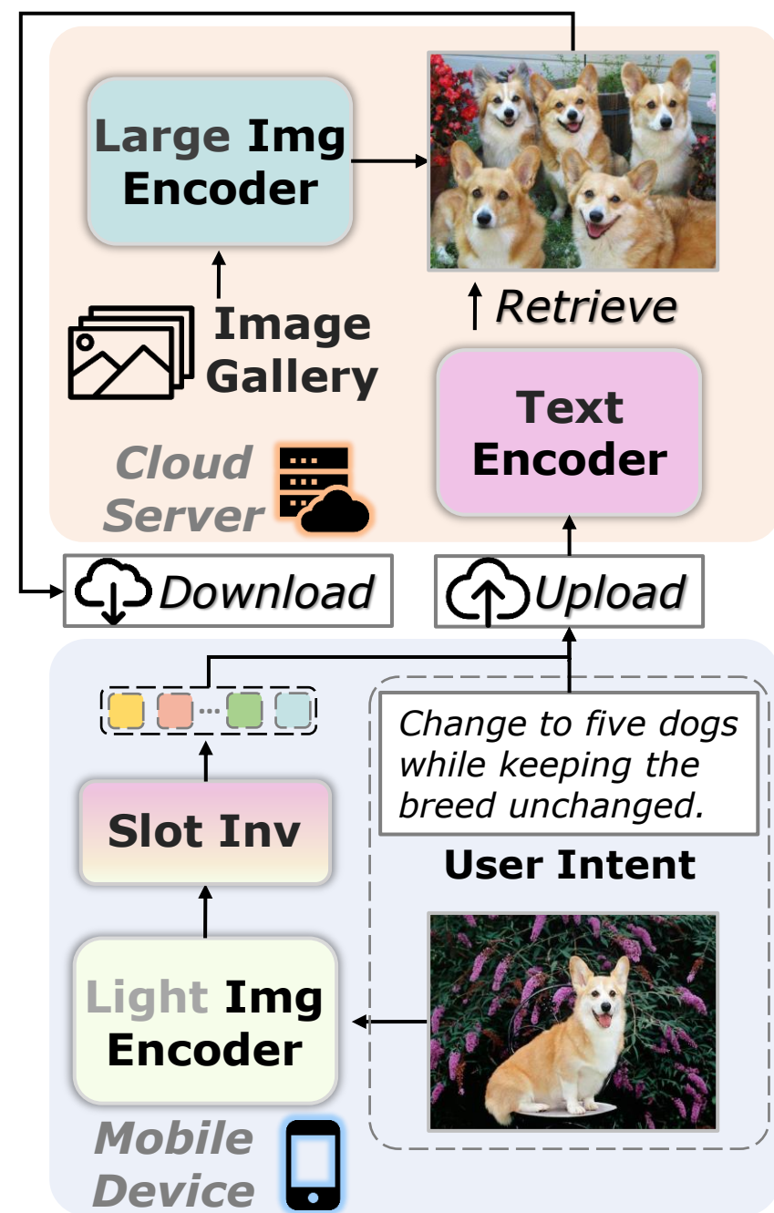
(b) The inference workflow
