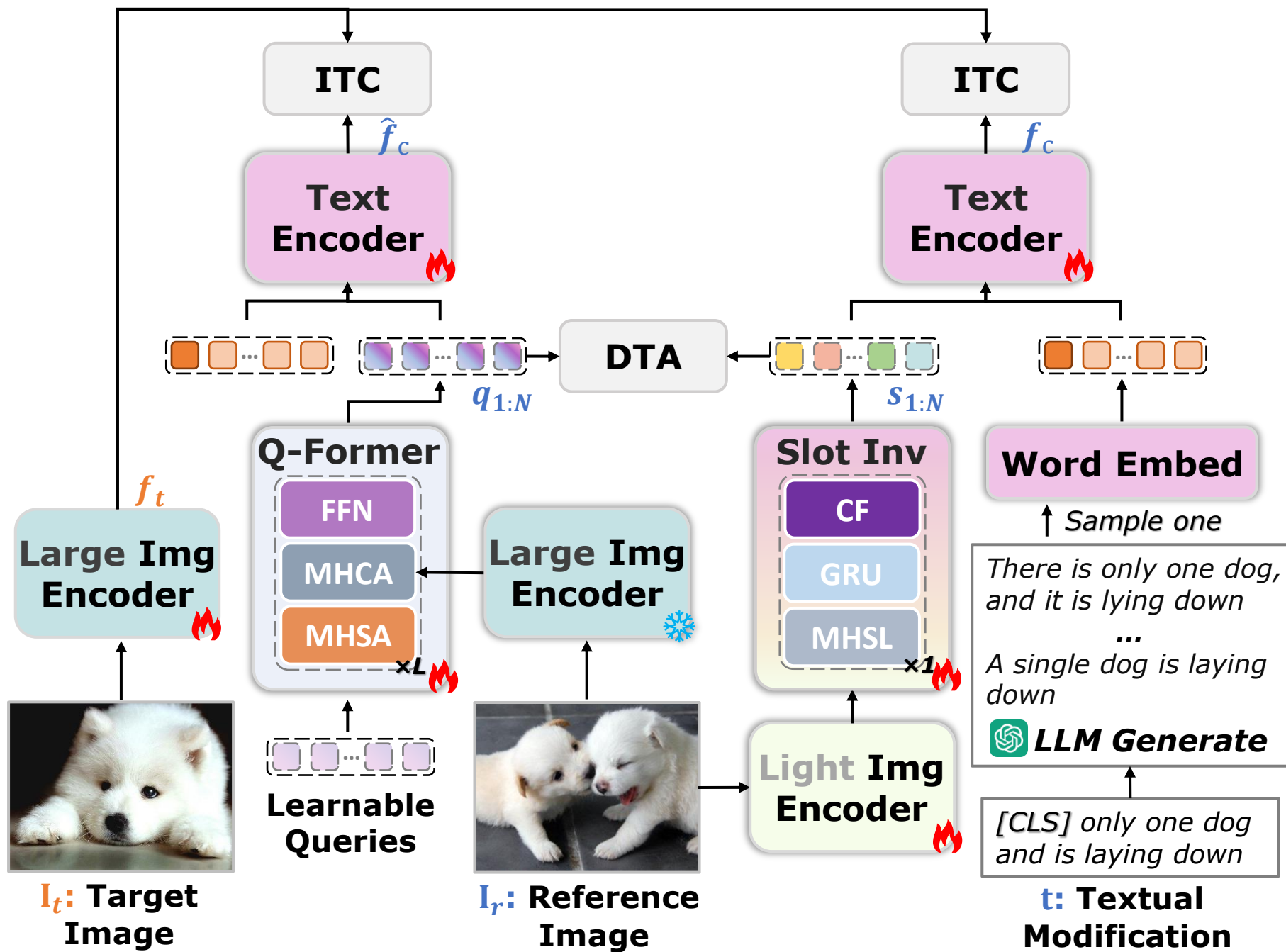
(a) Our training framework
