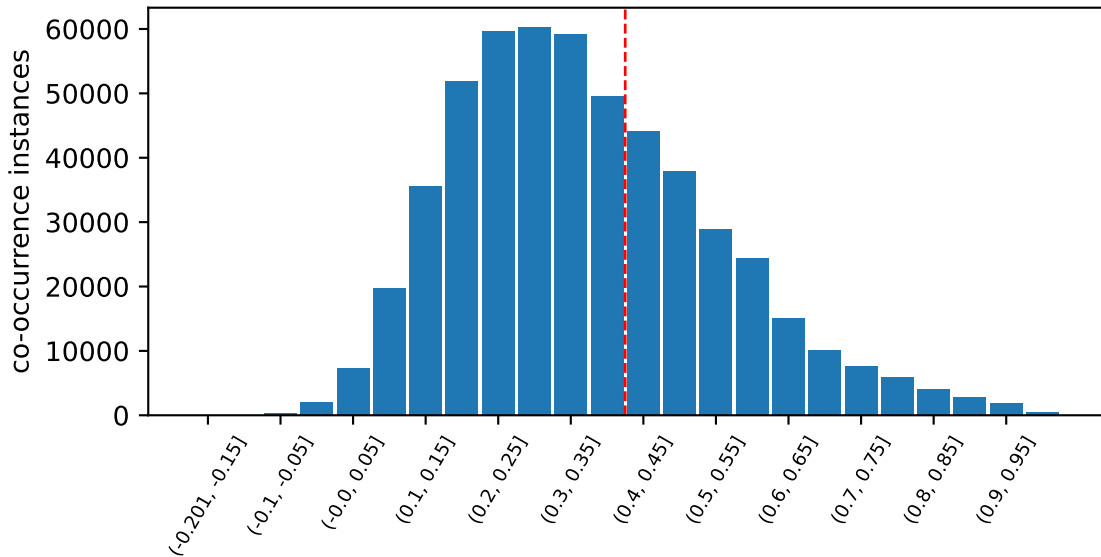
Cosine similarity of co-occurring keyword pairs
