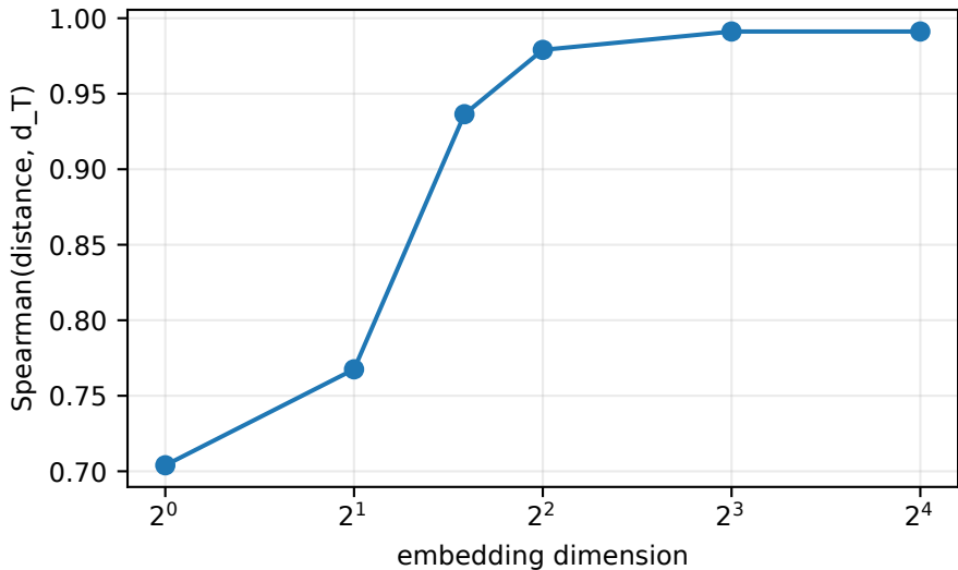
Transition-distance rank fidelity
