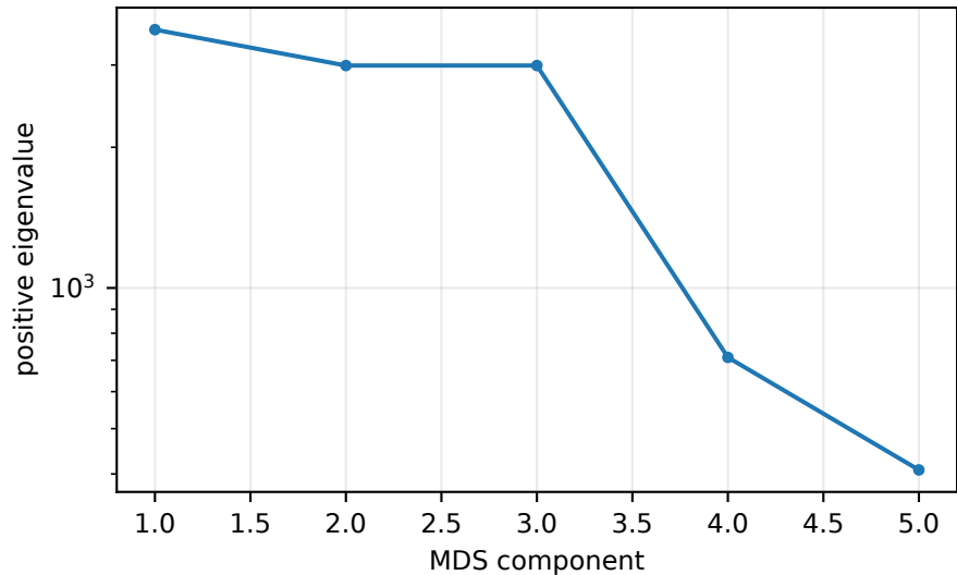
Controlled toy transition spectrum
