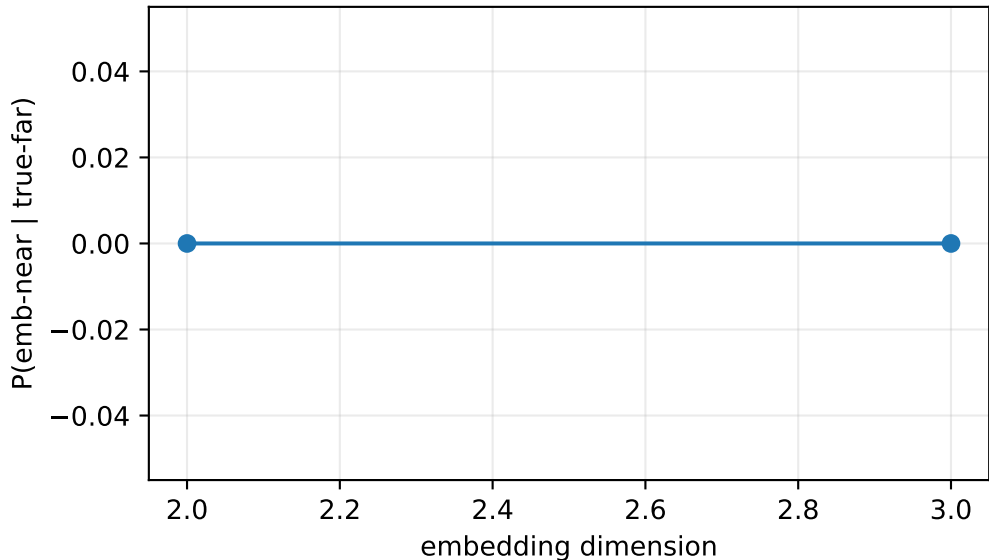
Crossroad false shortcuts vs dimension
