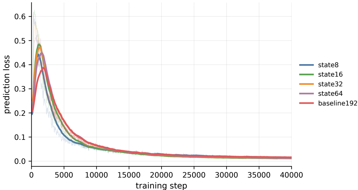
Prediction loss: no-bottleneck dimension sweep
