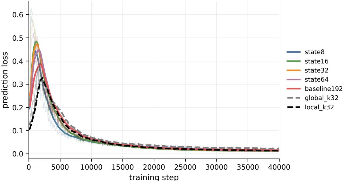
Prediction loss with bottleneck controls
