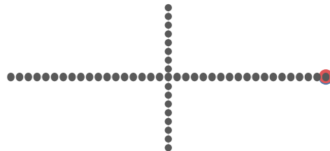
temporal_only
