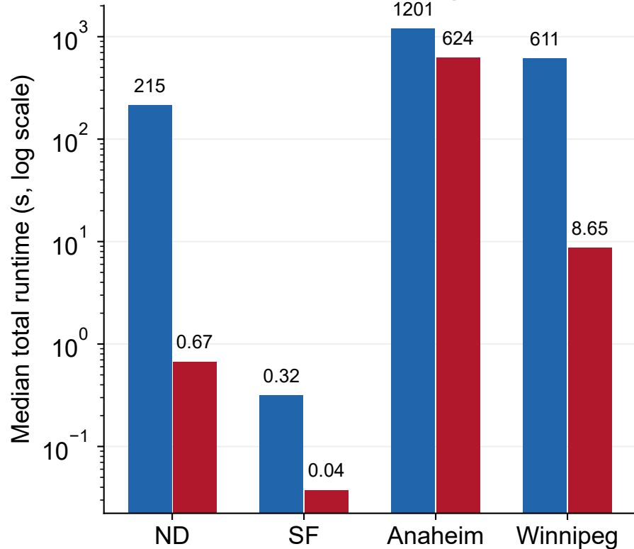
(b) Runtime under fixed stage limits
