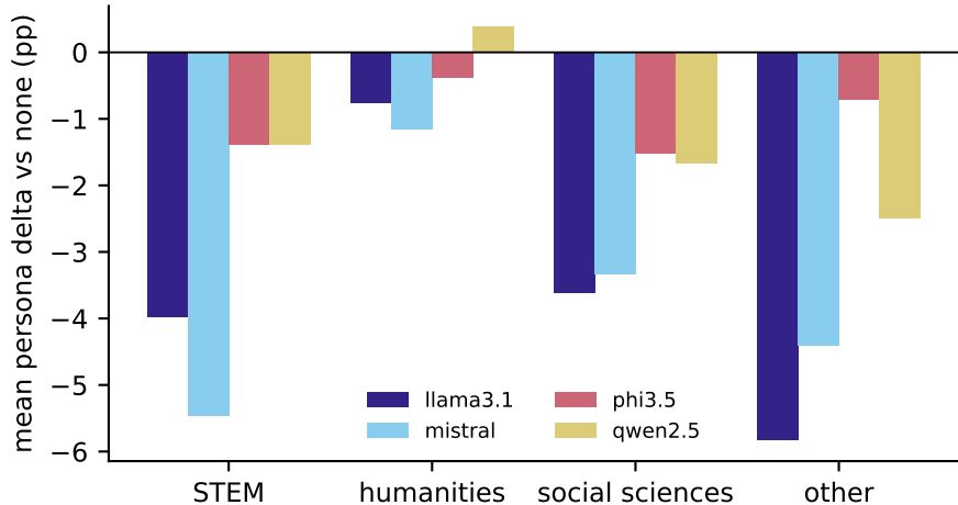
MMLU by domain
